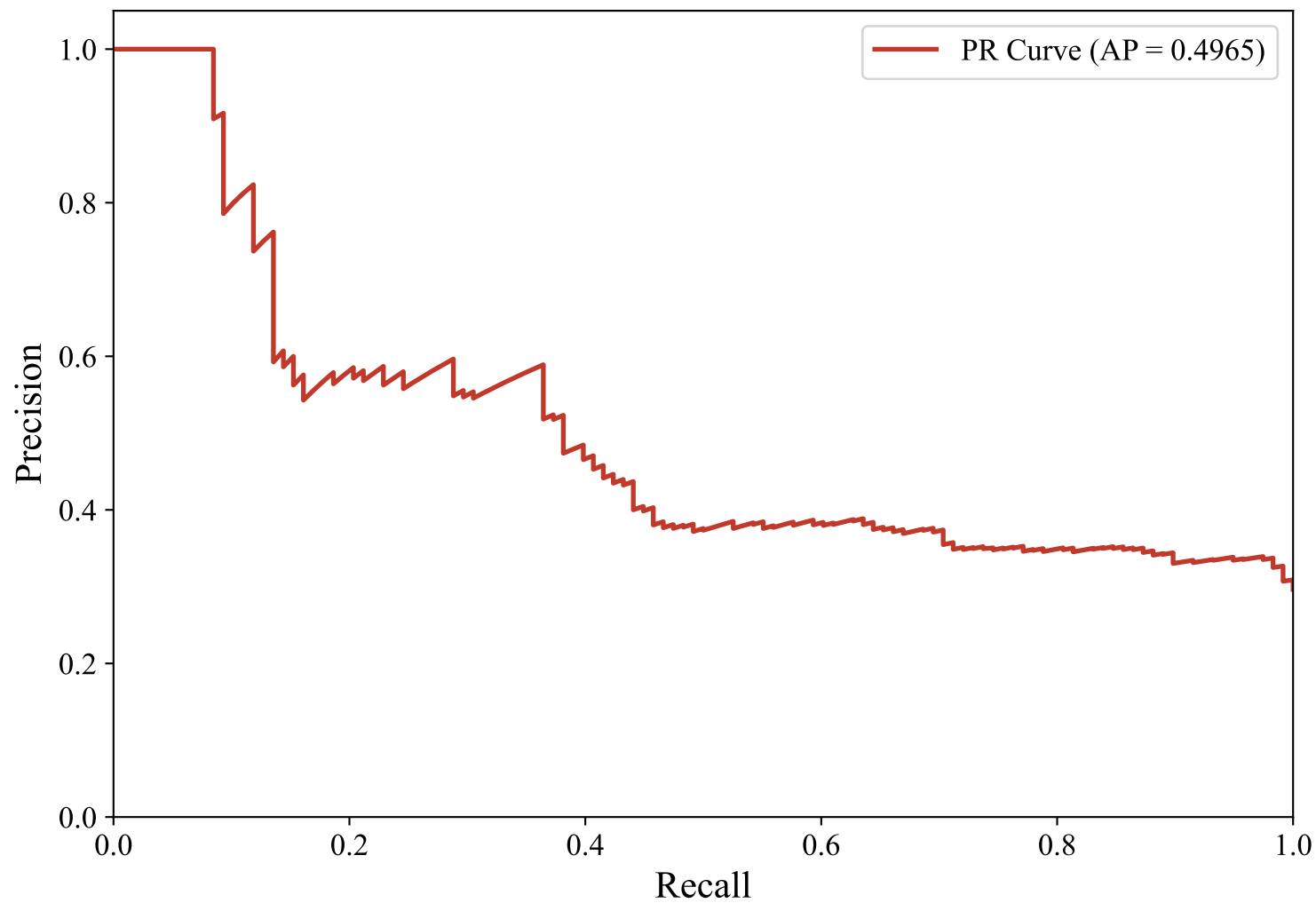
Precision-Recall Curve — DUTCH_MANUAL (multilingual-e5-large-instruct, svm_rbf)
