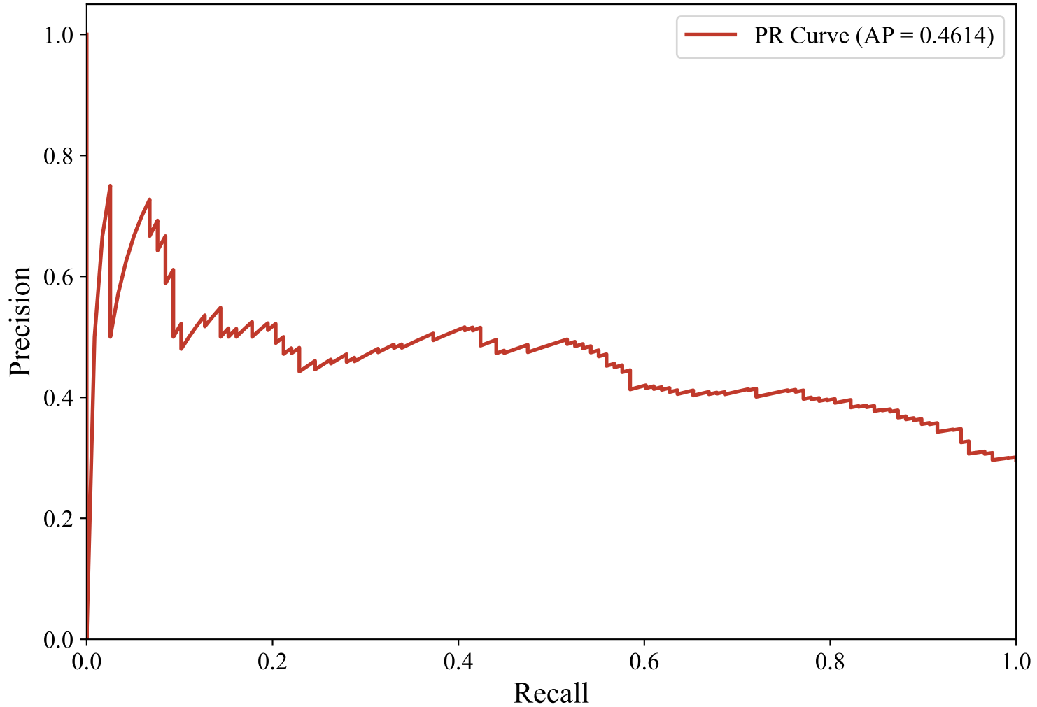
Precision-Recall Curve — DUTCH_MANUAL (paraphrase-multilingual-MiniLM-L12-v2, xgboost)
