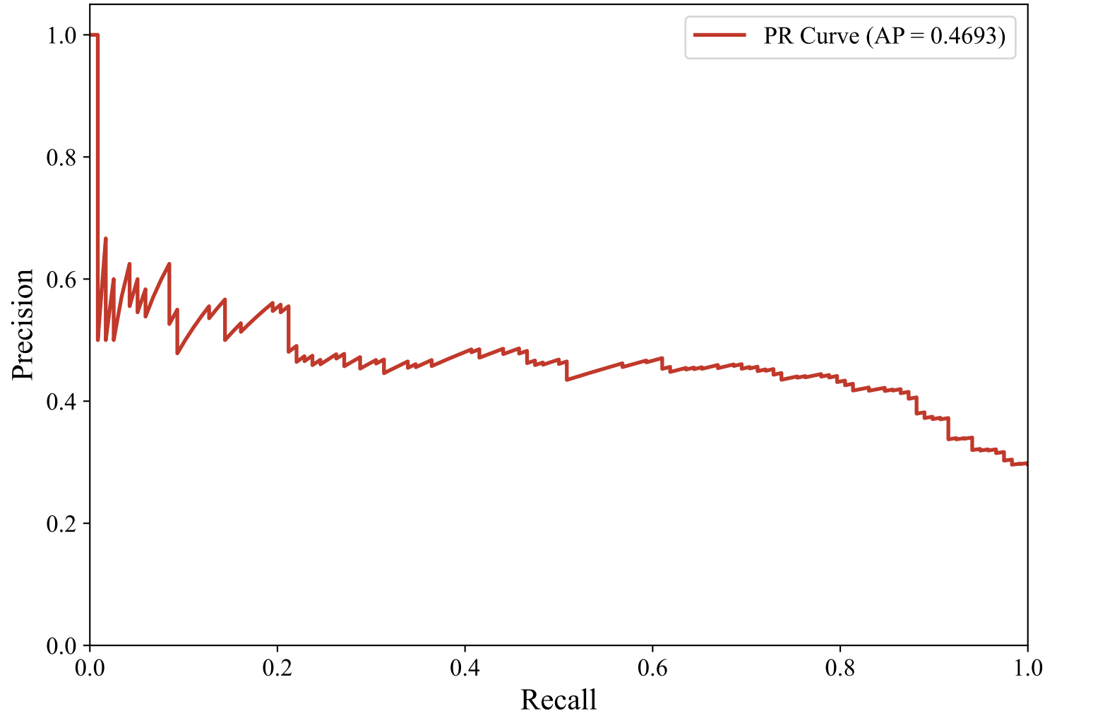
Precision-Recall Curve — DUTCH_MANUAL (paraphrase-multilingual-mpnet-base-v2, svm_linear)
