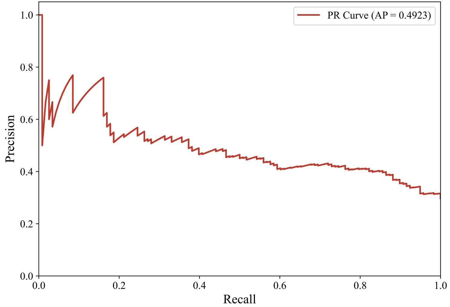
Precision-Recall Curve — DUTCH_MANUAL (snowflake-arctic-embed-l-v2.0, svm_linear)
