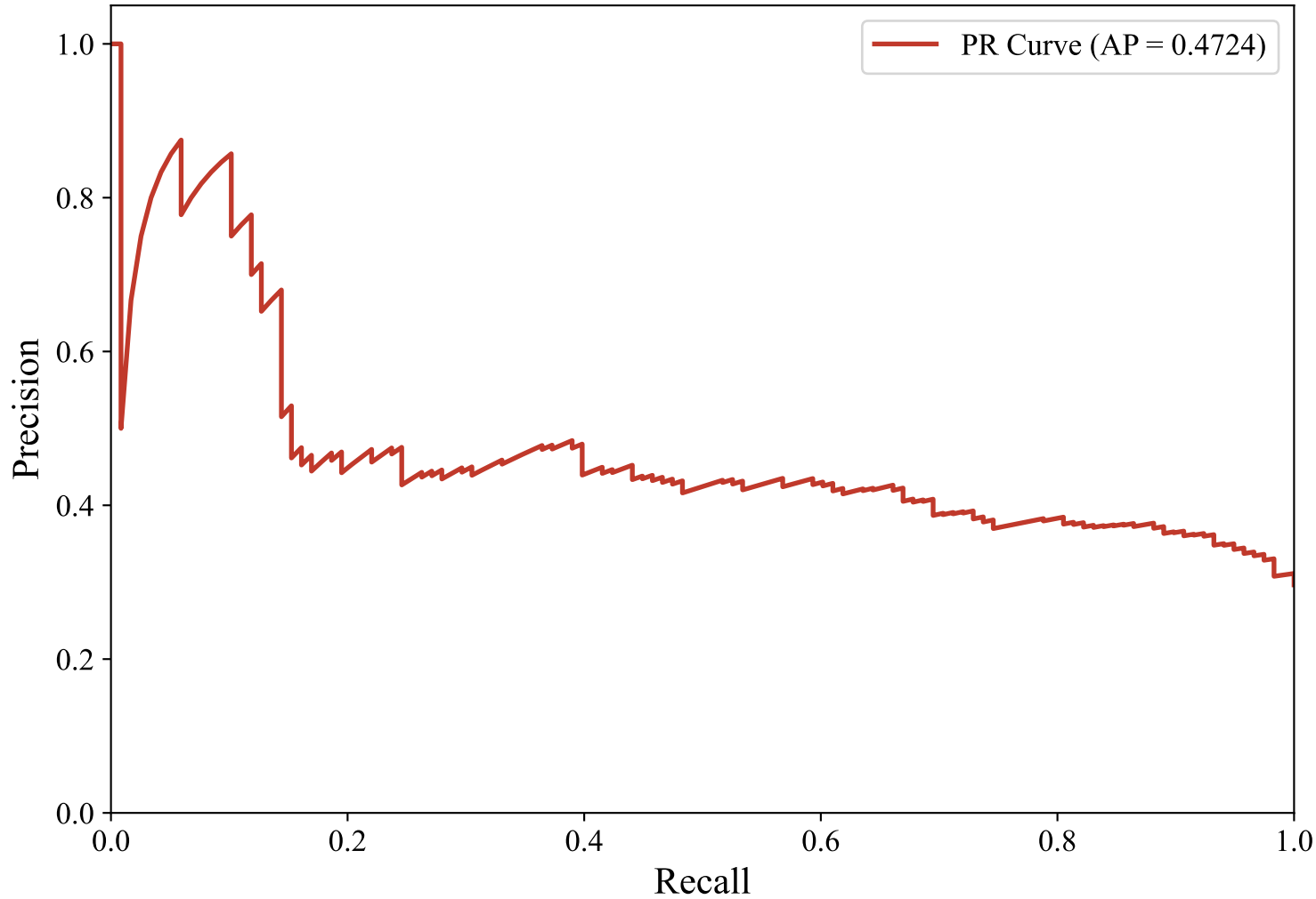
Precision-Recall Curve — DUTCH_MANUAL (xlm-roberta-base, svm_linear)
