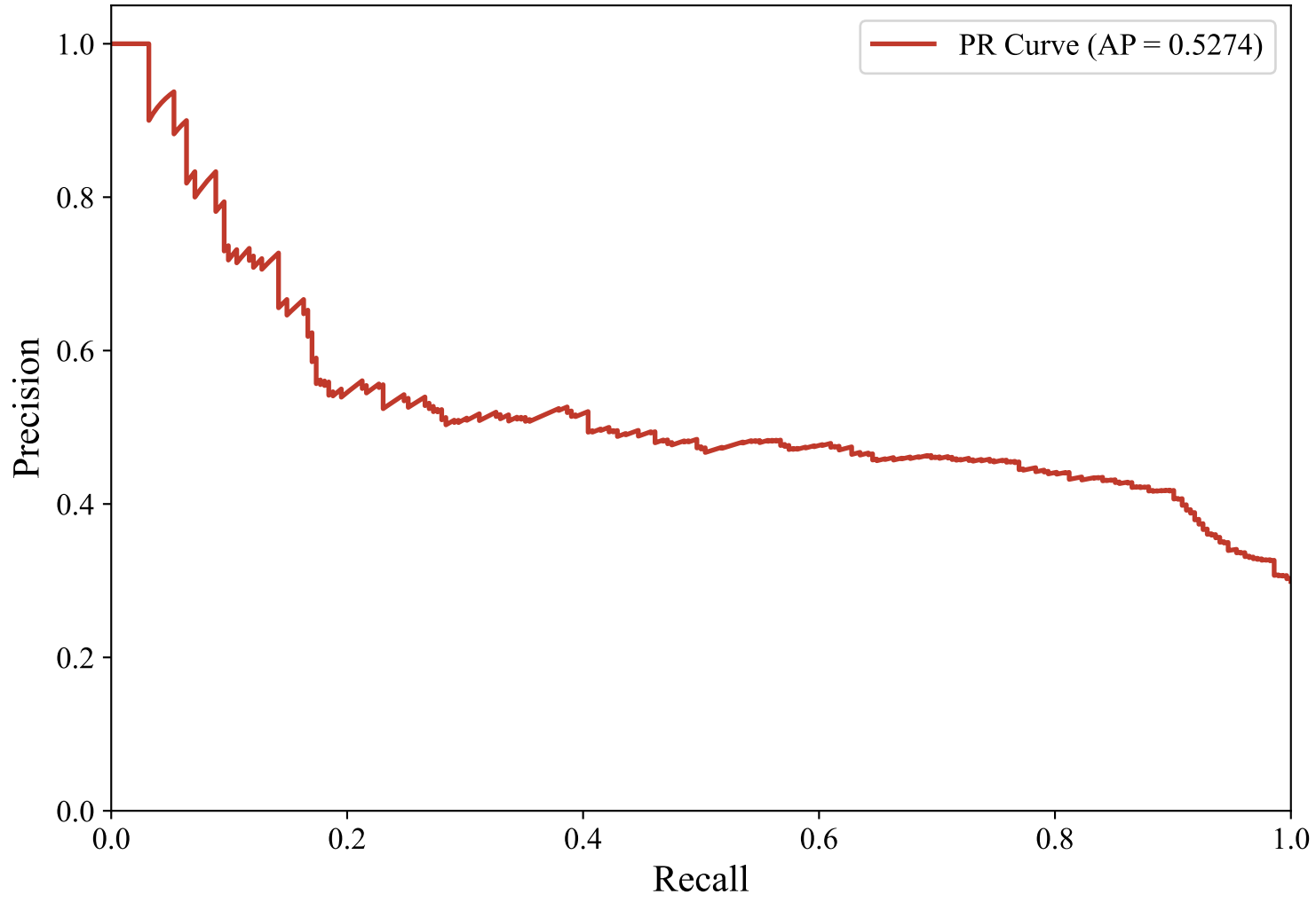
Precision-Recall Curve — ENGLISH_MANUAL (multilingual-e5-large-instruct, lightgbm)
