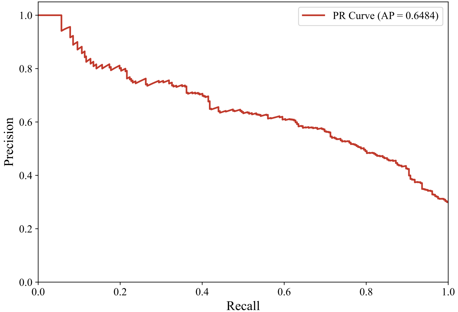
Precision-Recall Curve — ENGLISH_MANUAL (multilingual-e5-large-instruct, random_forest)
