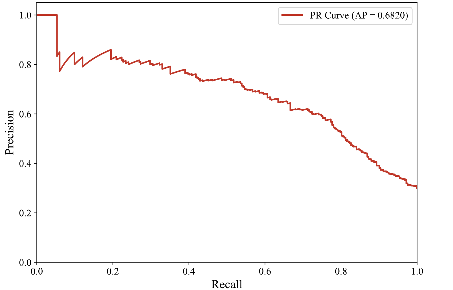
Precision-Recall Curve — ENGLISH_MANUAL (paraphrase-multilingual-MiniLM-L12-v2, random_forest)
