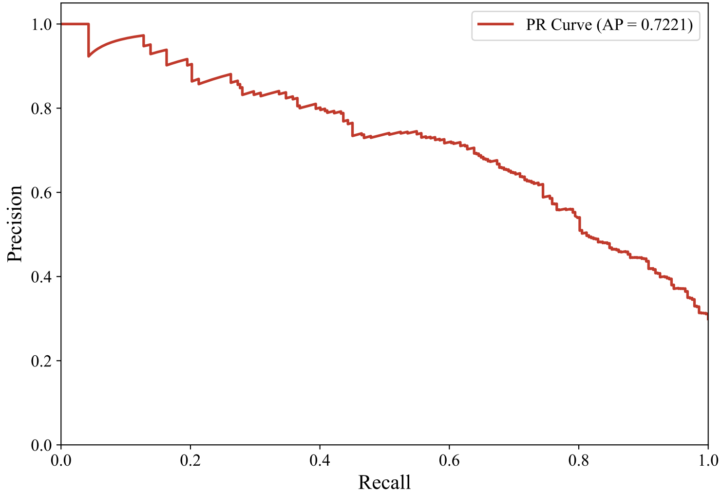
Precision-Recall Curve — ENGLISH_MANUAL (paraphrase-multilingual-MiniLM-L12-v2, svm_rbf)
