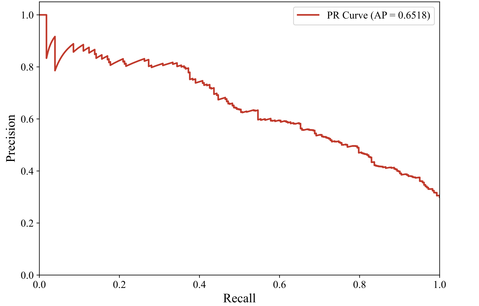
Precision-Recall Curve — ENGLISH_MANUAL (paraphrase-multilingual-MiniLM-L12-v2, xgboost)
