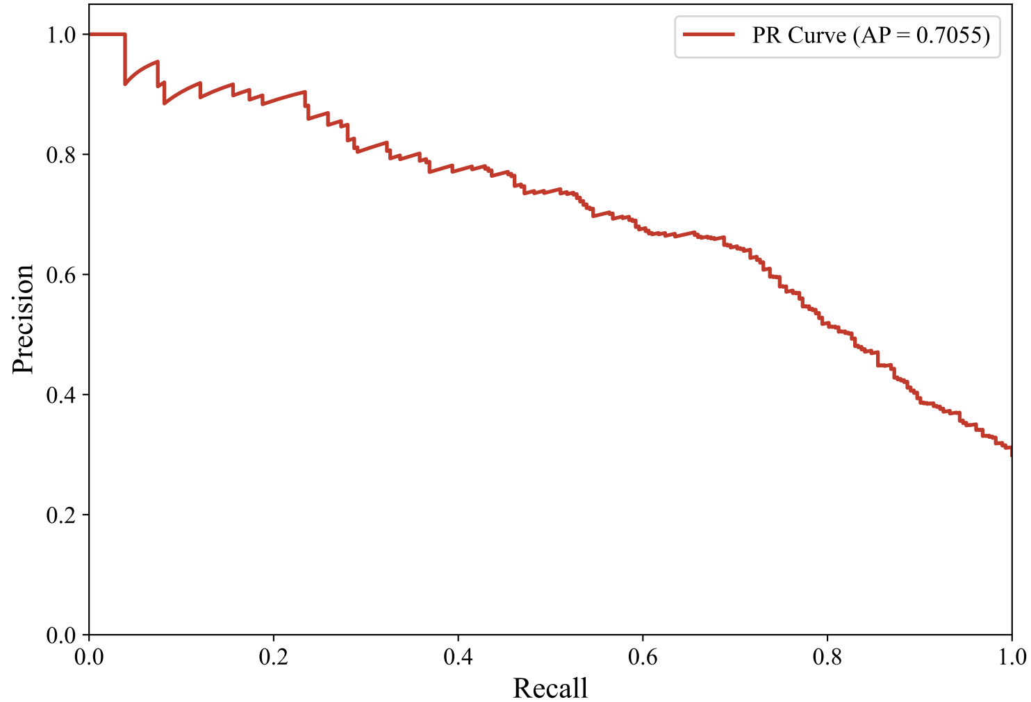
Precision-Recall Curve — ENGLISH_MANUAL (paraphrase-multilingual-mpnet-base-v2, random_forest)
