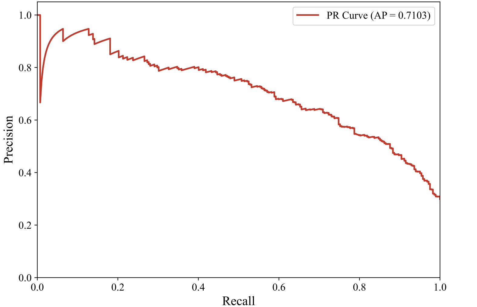
Precision-Recall Curve — ENGLISH_MANUAL (paraphrase-multilingual-mpnet-base-v2, svm_rbf)
