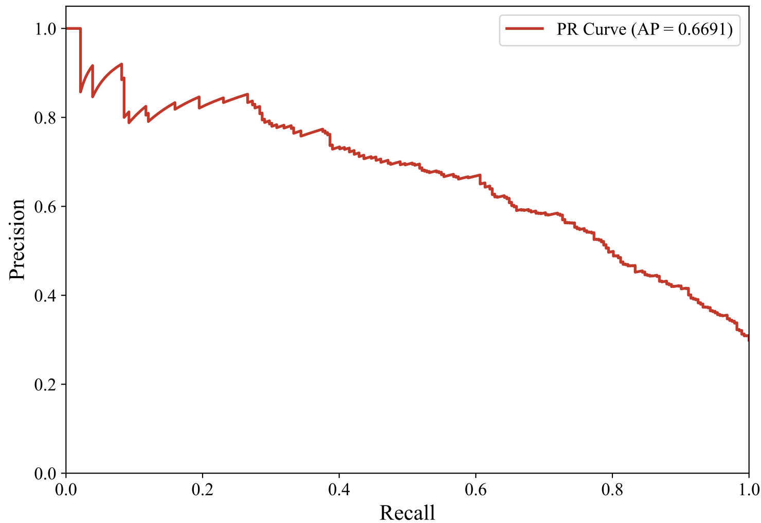
Precision-Recall Curve — ENGLISH_MANUAL (paraphrase-multilingual-mpnet-base-v2, xgboost)
