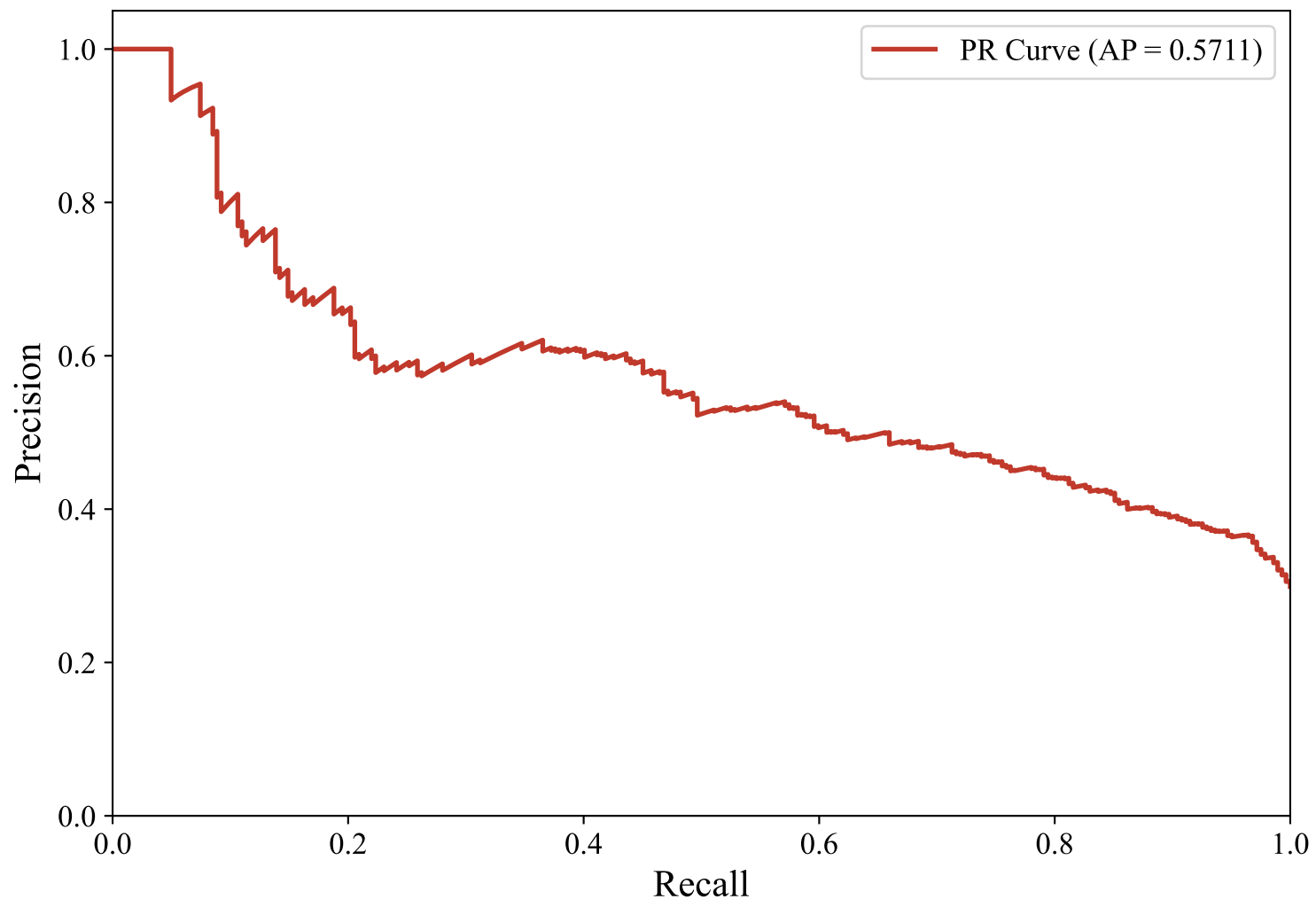
Precision-Recall Curve — ENGLISH_MANUAL (snowflake-arctic-embed-l-v2.0, svm_linear)
