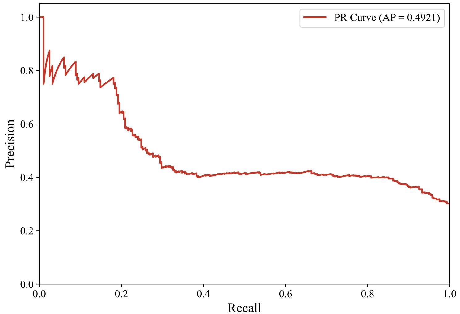
Precision-Recall Curve — ENGLISH_MANUAL (snowflake-arctic-embed-l-v2.0, xgboost)
