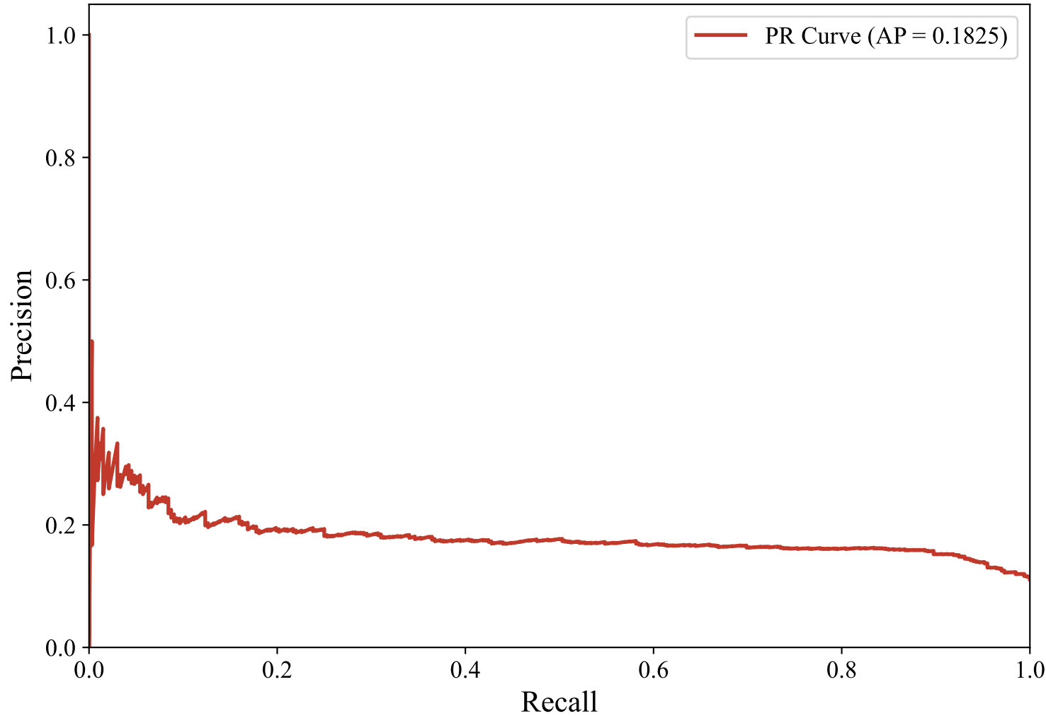
Precision-Recall Curve — GERMAN_MANUAL (bert-base-multilingual-uncased, random_forest)
