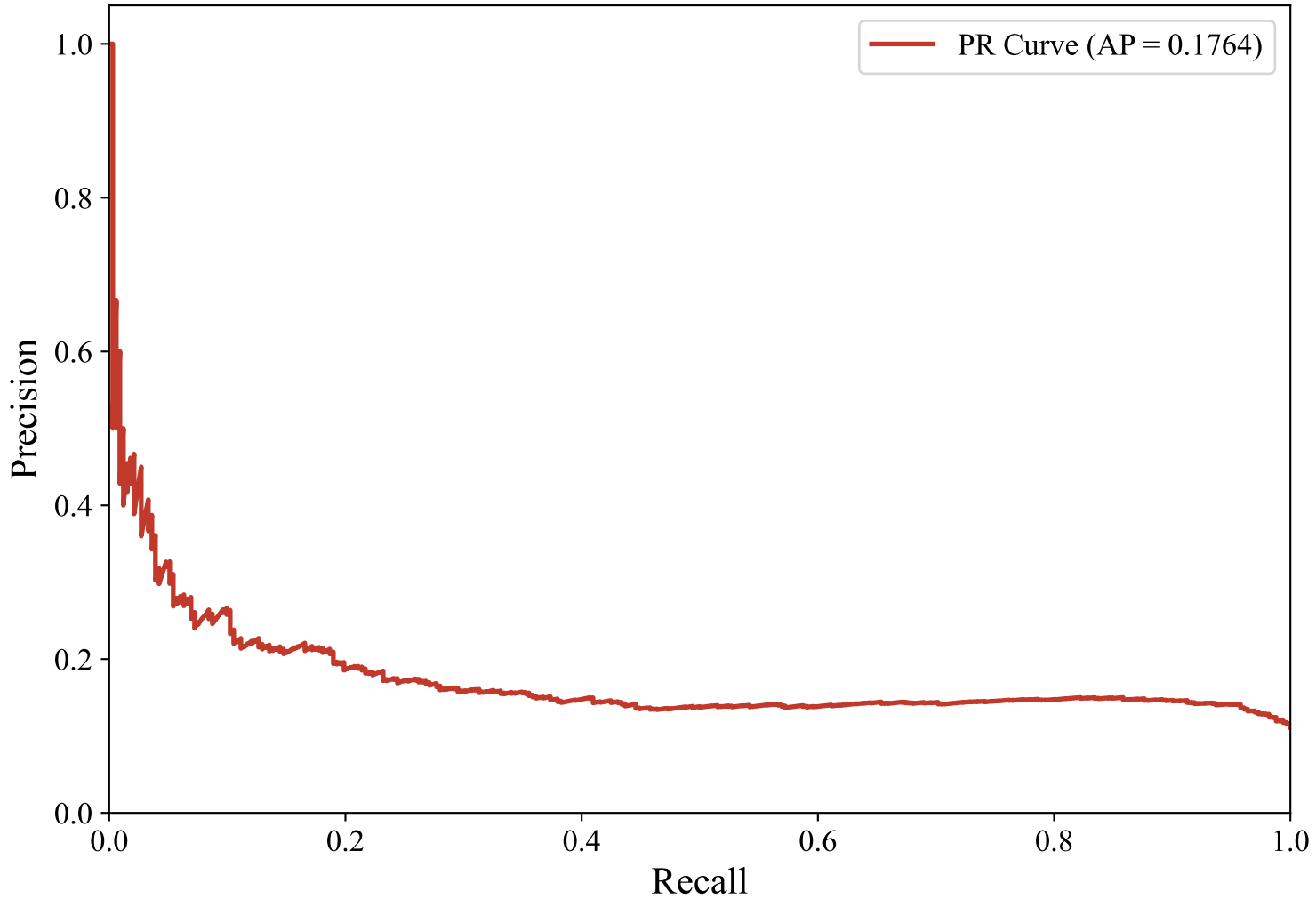
Precision-Recall Curve — GERMAN_MANUAL (multilingual-e5-large-instruct, xgboost)
