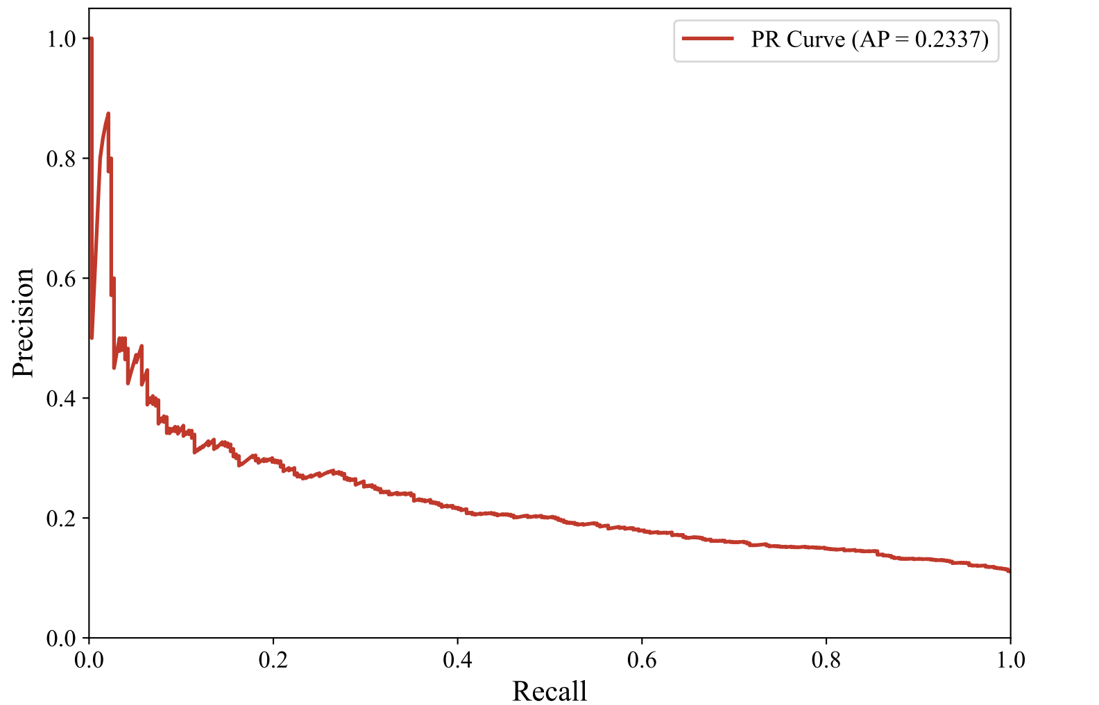
Precision-Recall Curve — GERMAN_MANUAL (paraphrase-multilingual-MiniLM-L12-v2, random_forest)
