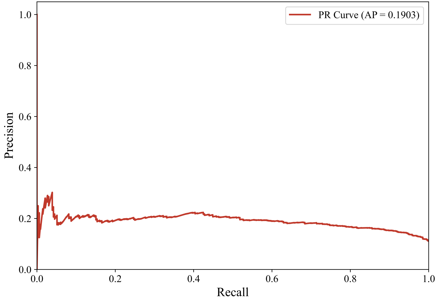
Precision-Recall Curve — GERMAN_MANUAL (paraphrase-multilingual-MiniLM-L12-v2, svm_rbf)
