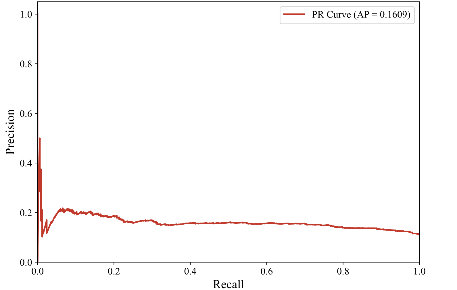
Precision-Recall Curve — GERMAN_MANUAL (paraphrase-multilingual-MiniLM-L12-v2, xgboost)
