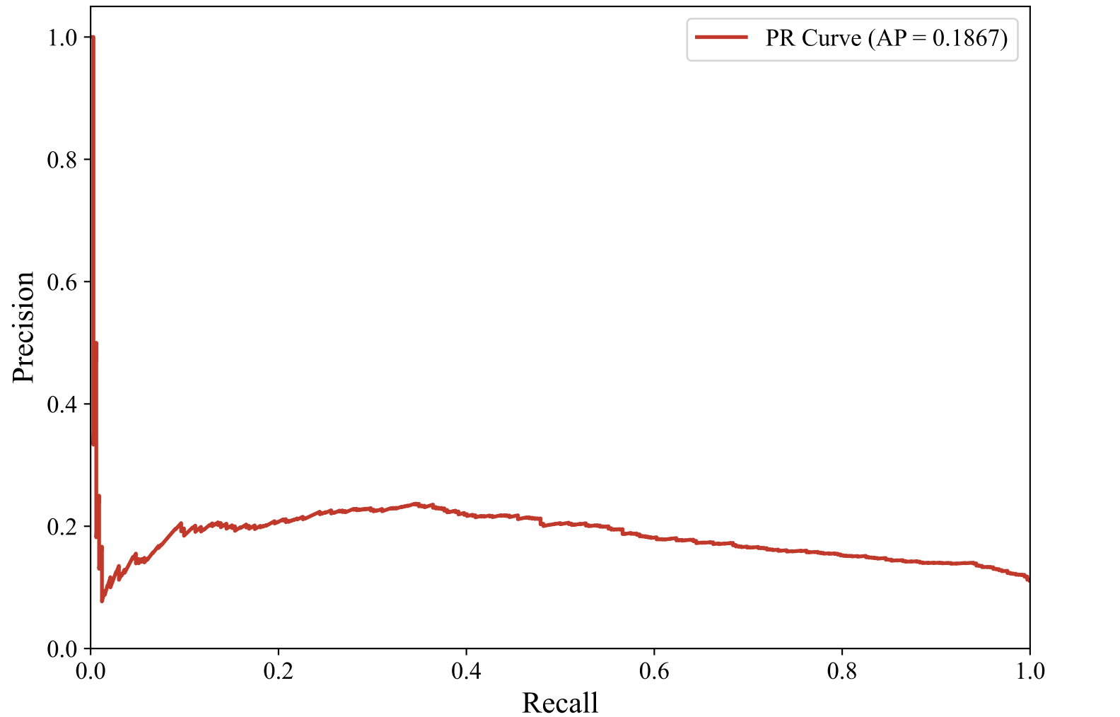
Precision-Recall Curve — GERMAN_MANUAL (paraphrase-multilingual-mpnet-base-v2, random_forest)
