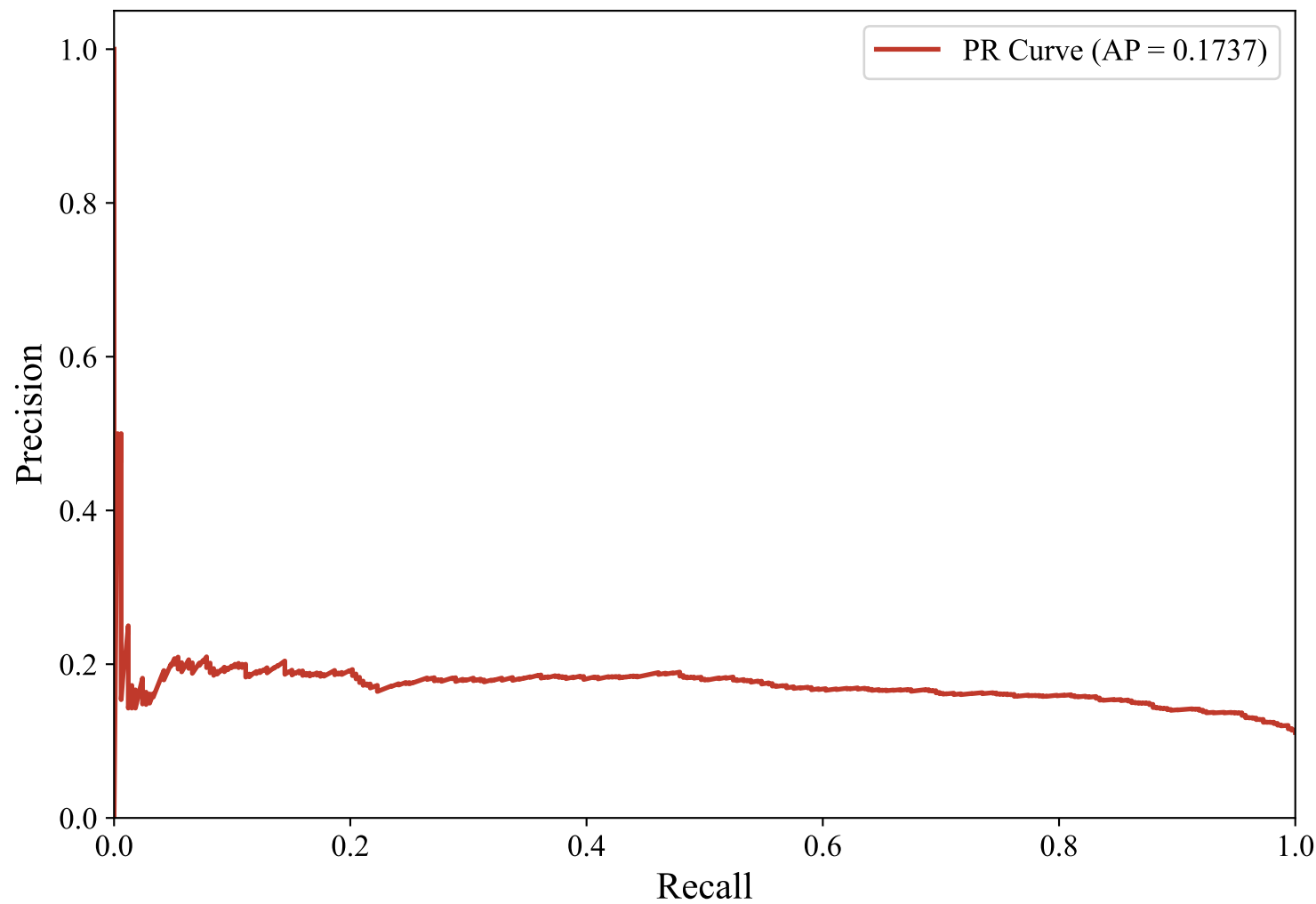
Precision-Recall Curve — GERMAN_MANUAL (paraphrase-multilingual-mpnet-base-v2, xgboost)
