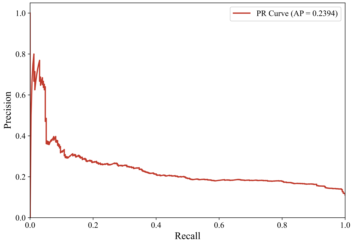
Precision-Recall Curve — GERMAN_MANUAL (snowflake-arctic-embed-l-v2.0, svm_linear)
