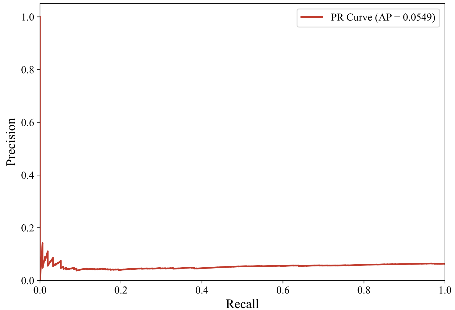
Precision-Recall Curve — SWEDISH_MANUAL (bert-base-multilingual-uncased, lightgbm)
