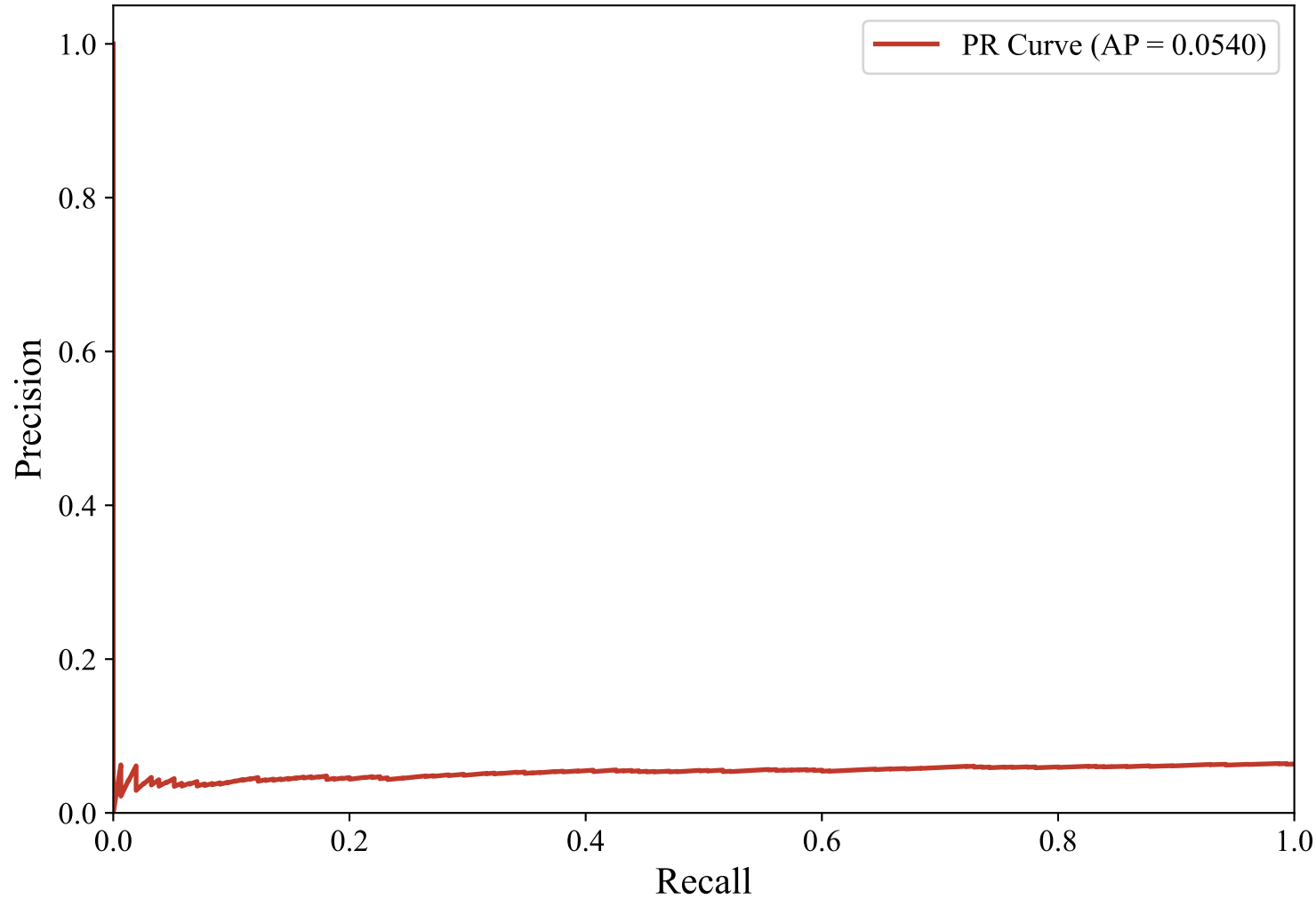
Precision-Recall Curve — SWEDISH_MANUAL (bert-base-multilingual-uncased, random_forest)
