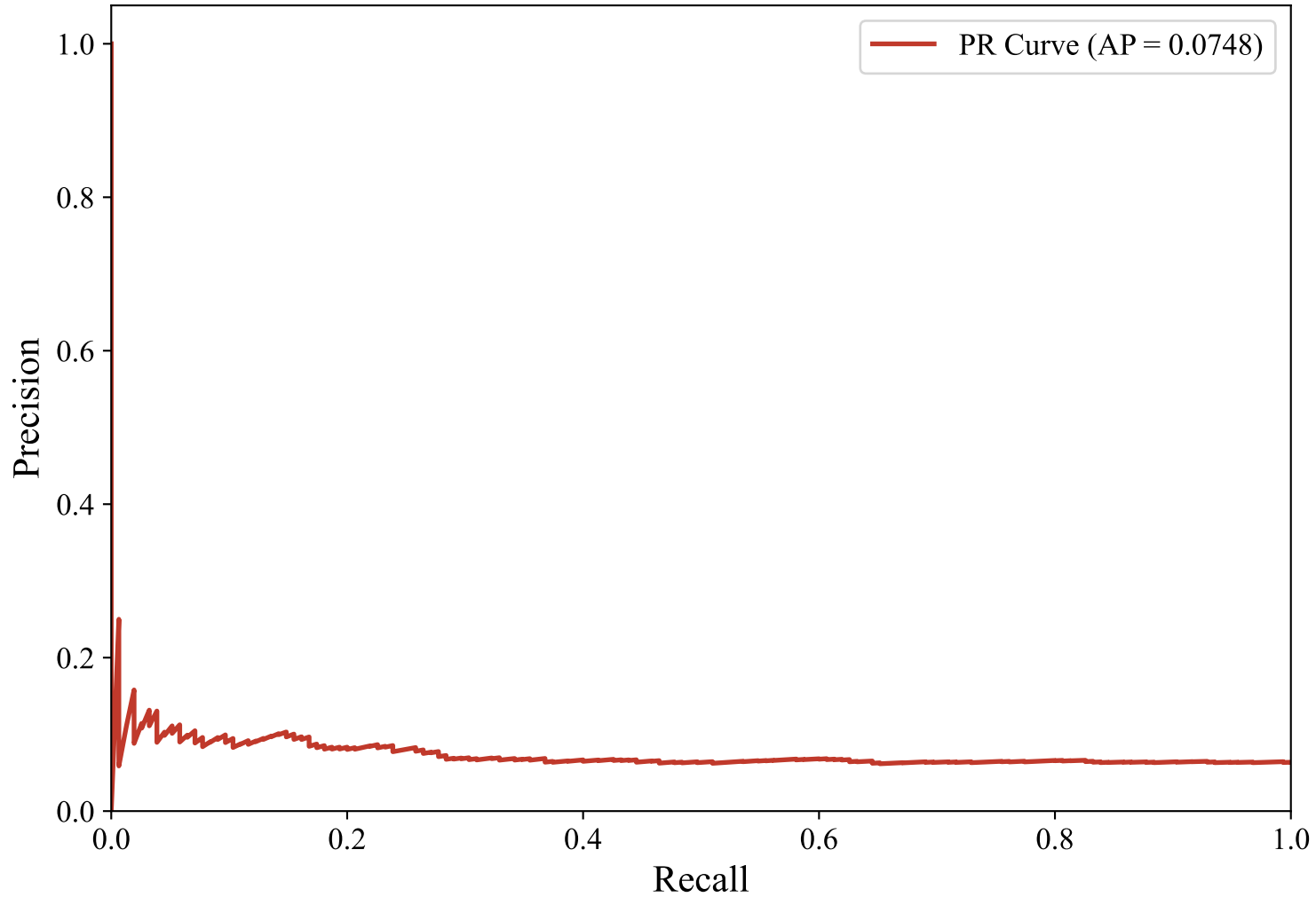
Precision-Recall Curve — SWEDISH_MANUAL (bert-base-multilingual-uncased, svm_rbf)
