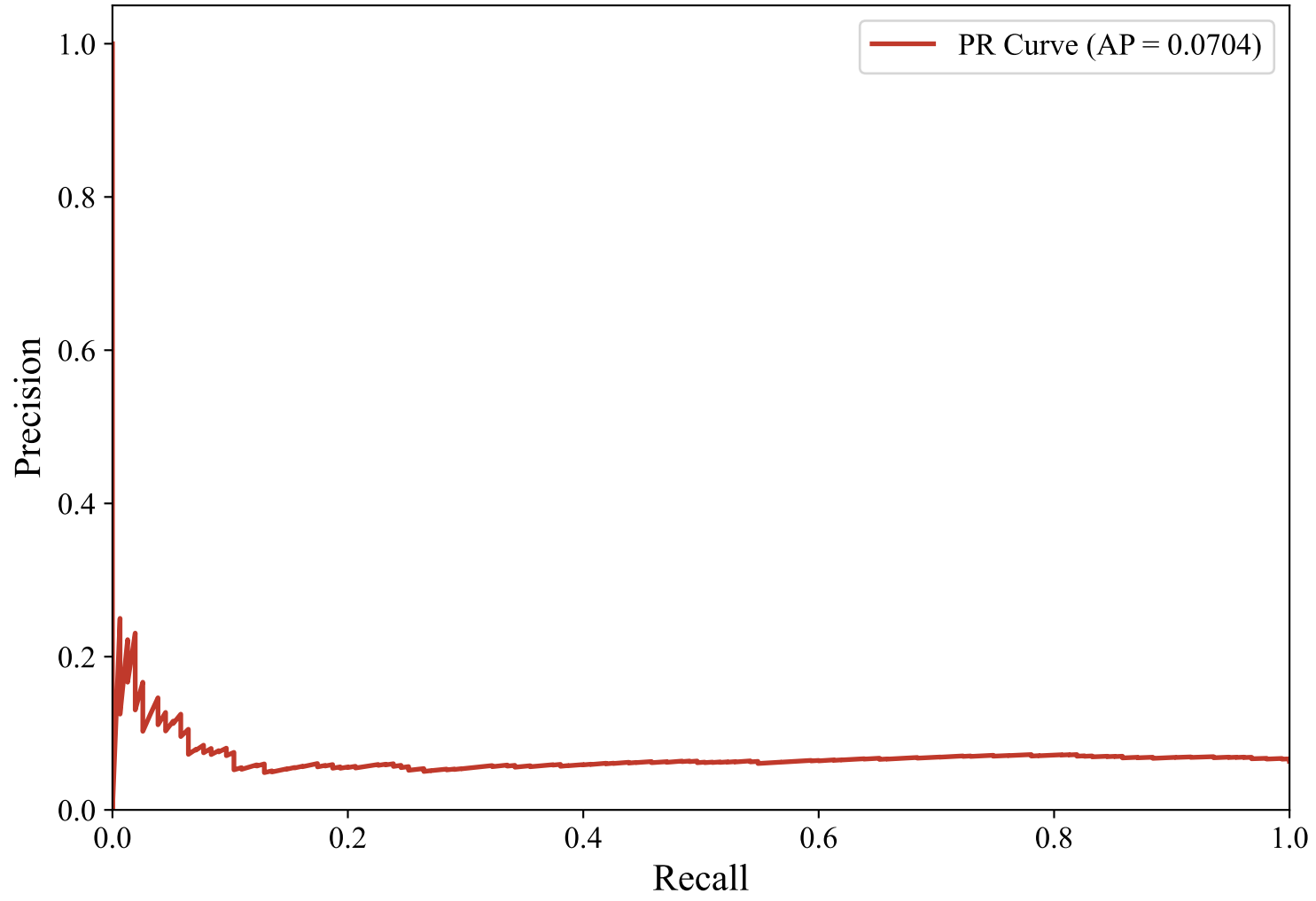
Precision-Recall Curve — SWEDISH_MANUAL (multilingual-e5-large-instruct, lightgbm)
