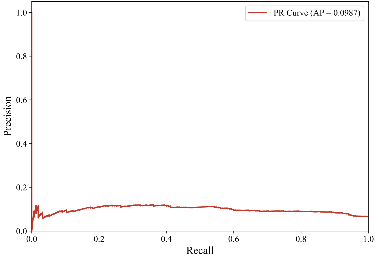
Precision-Recall Curve — SWEDISH_MANUAL (multilingual-e5-large-instruct, svm_linear)
