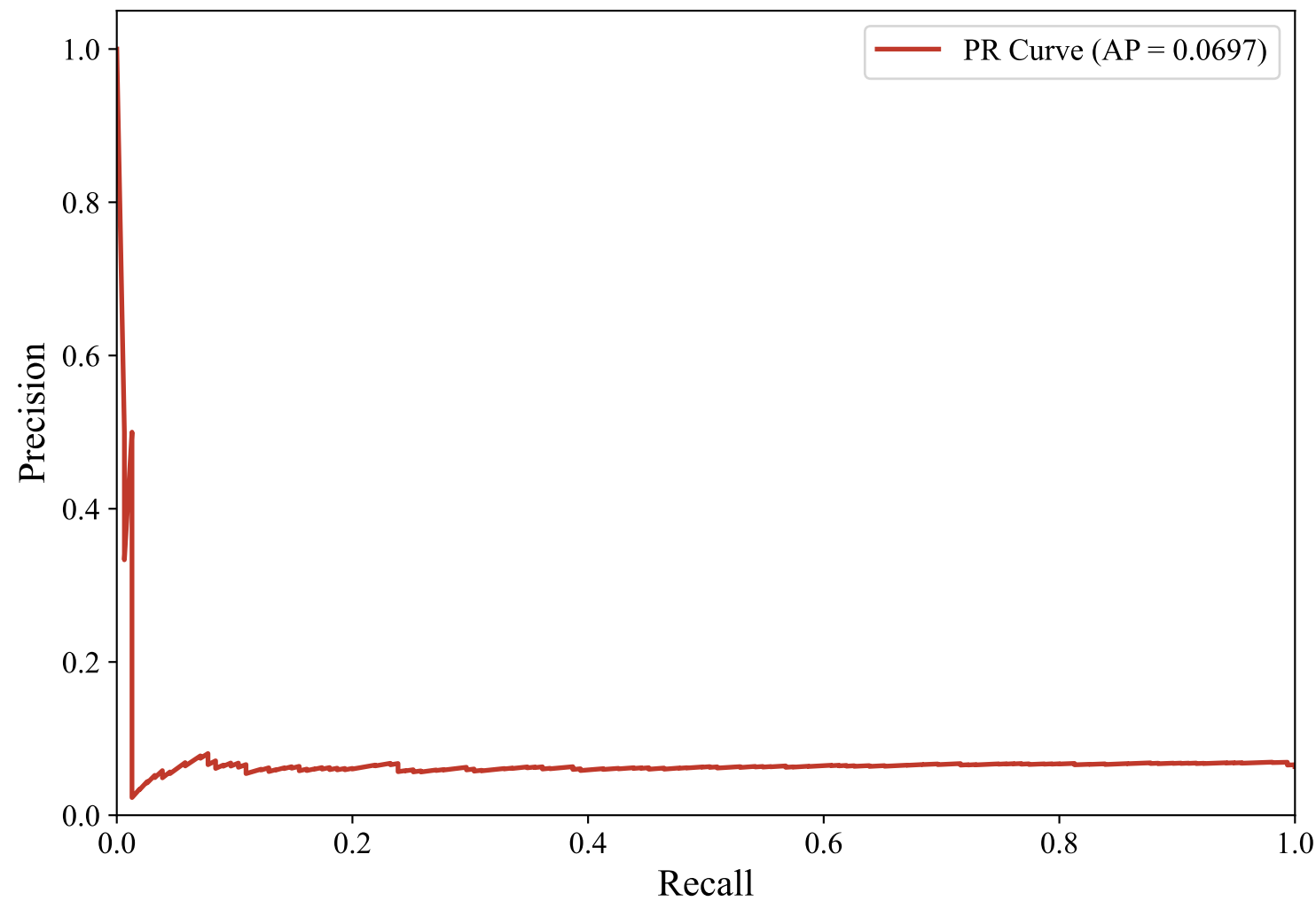
Precision-Recall Curve — SWEDISH_MANUAL (paraphrase-multilingual-MiniLM-L12-v2, lightgbm)
