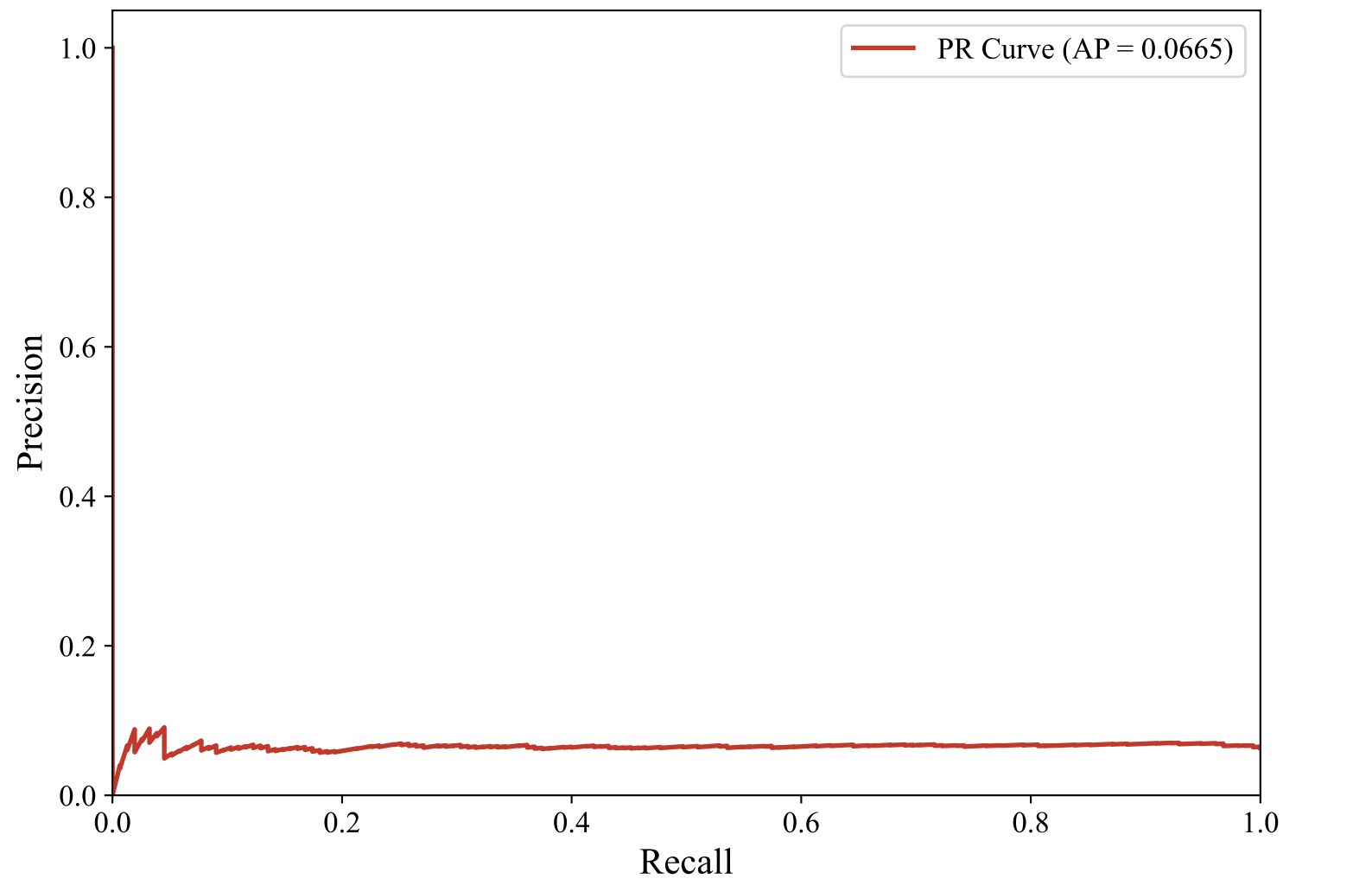
Precision-Recall Curve — SWEDISH_MANUAL (paraphrase-multilingual-MiniLM-L12-v2, random_forest)
