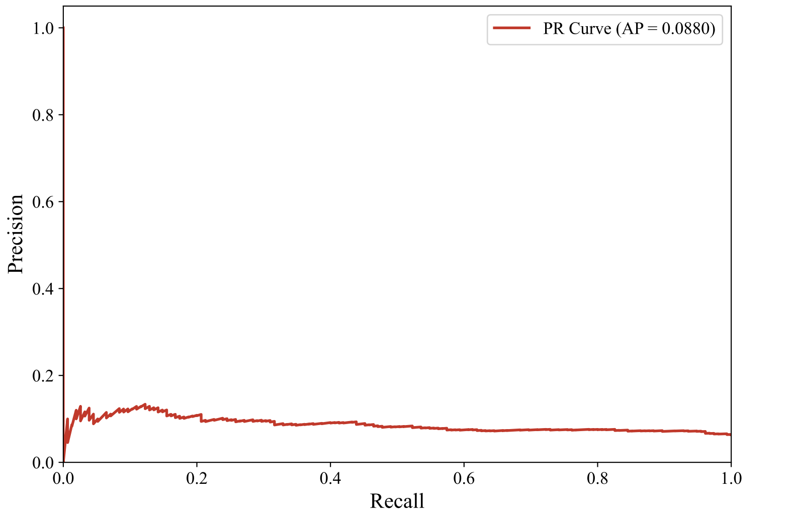
Precision-Recall Curve — SWEDISH_MANUAL (paraphrase-multilingual-MiniLM-L12-v2, svm_linear)
