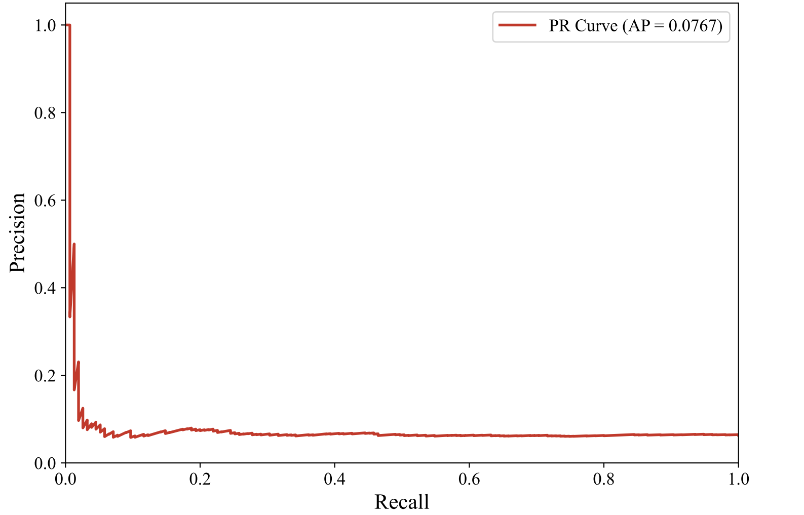
Precision-Recall Curve — SWEDISH_MANUAL (paraphrase-multilingual-mpnet-base-v2, lightgbm)
