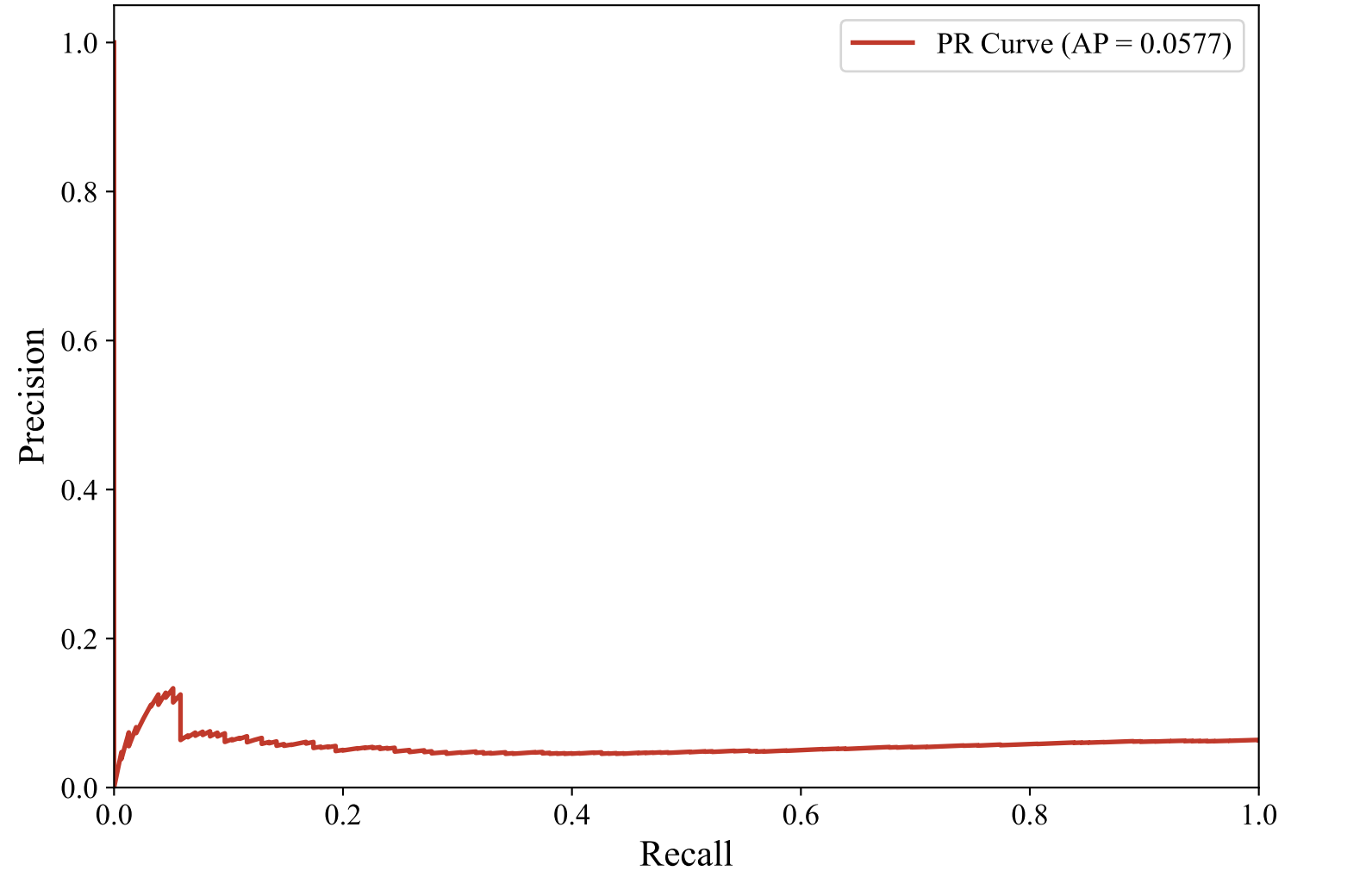
Precision-Recall Curve — SWEDISH_MANUAL (xlm-roberta-base, xgboost)
