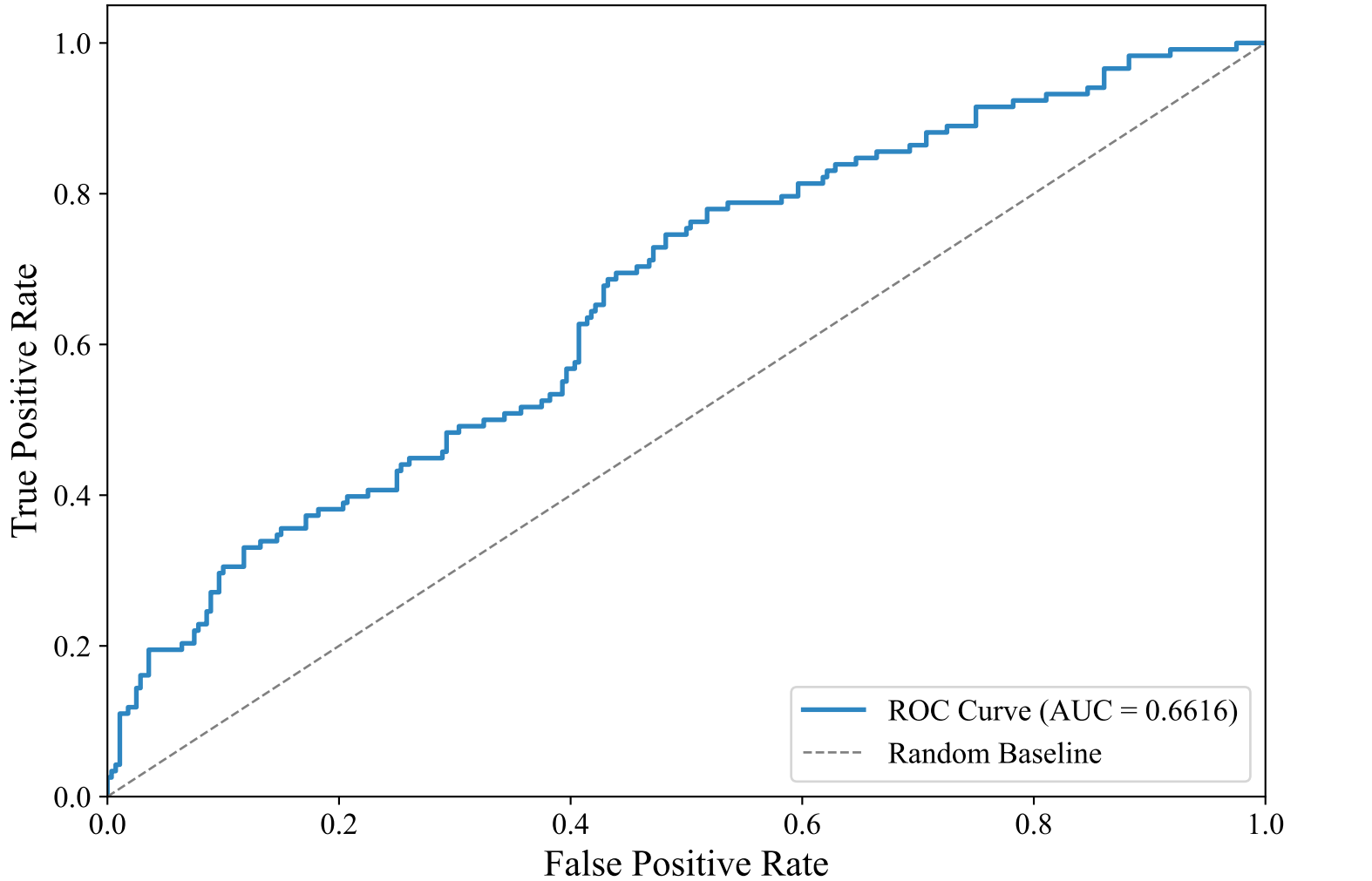
ROC Curve — DUTCH_MANUAL (multilingual-e5-large-instruct, random_forest)
