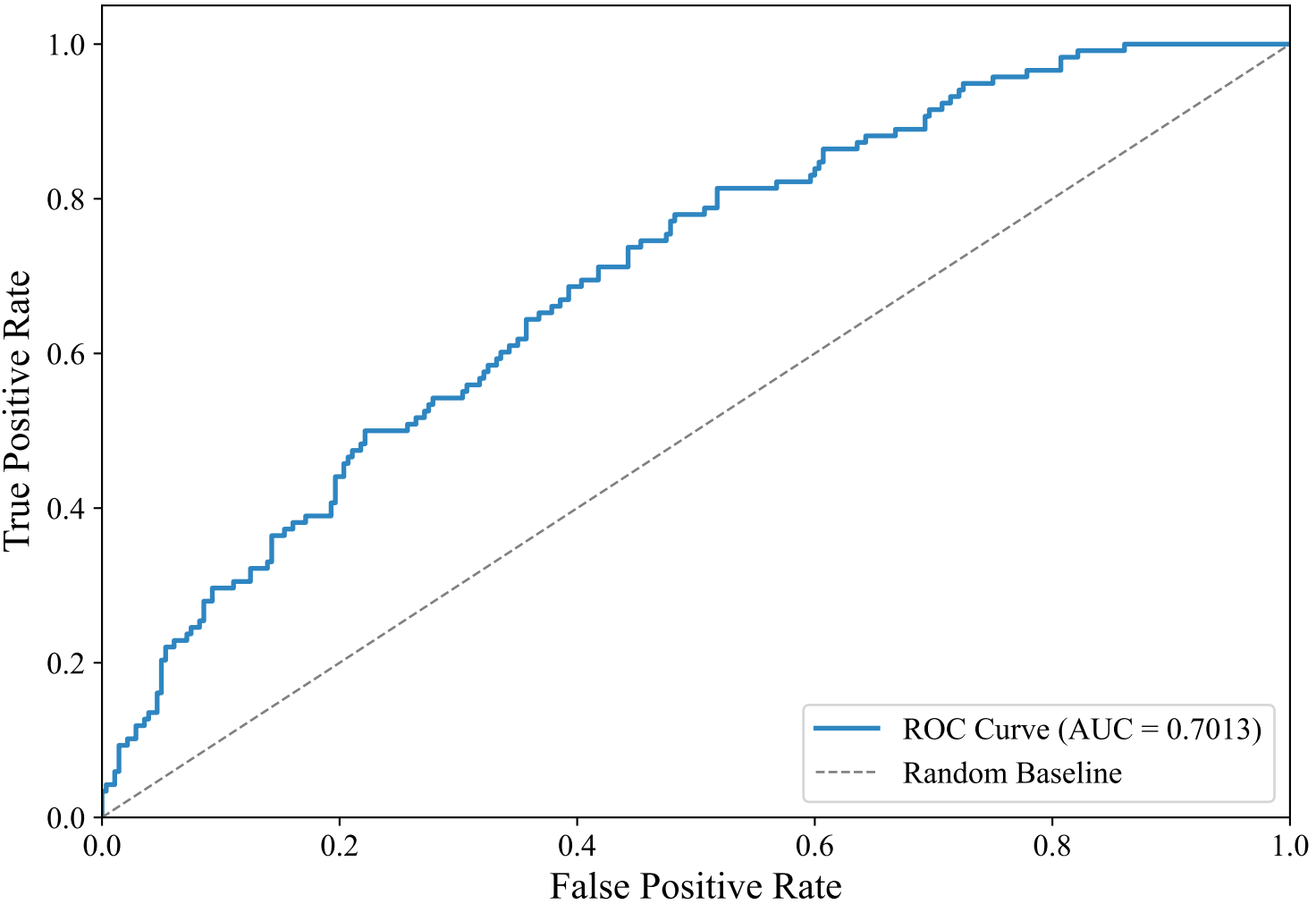
ROC Curve — DUTCH_MANUAL (multilingual-e5-large-instruct, svm_linear)
