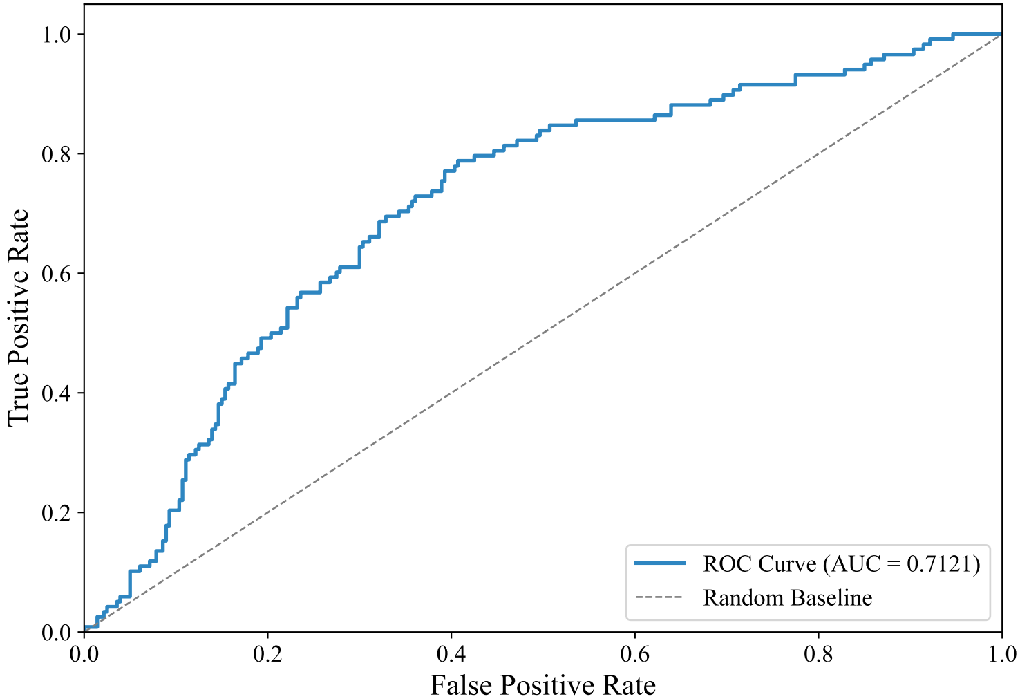
ROC Curve — DUTCH_MANUAL (paraphrase-multilingual-MiniLM-L12-v2, svm_linear)
