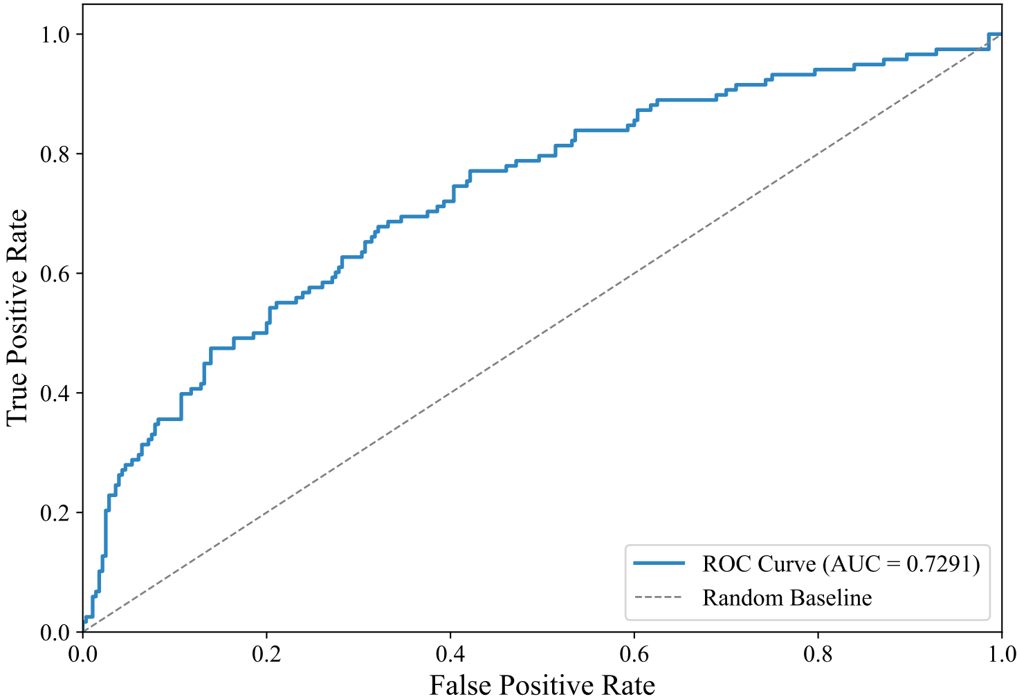
ROC Curve — DUTCH_MANUAL (paraphrase-multilingual-mpnet-base-v2, random_forest)
