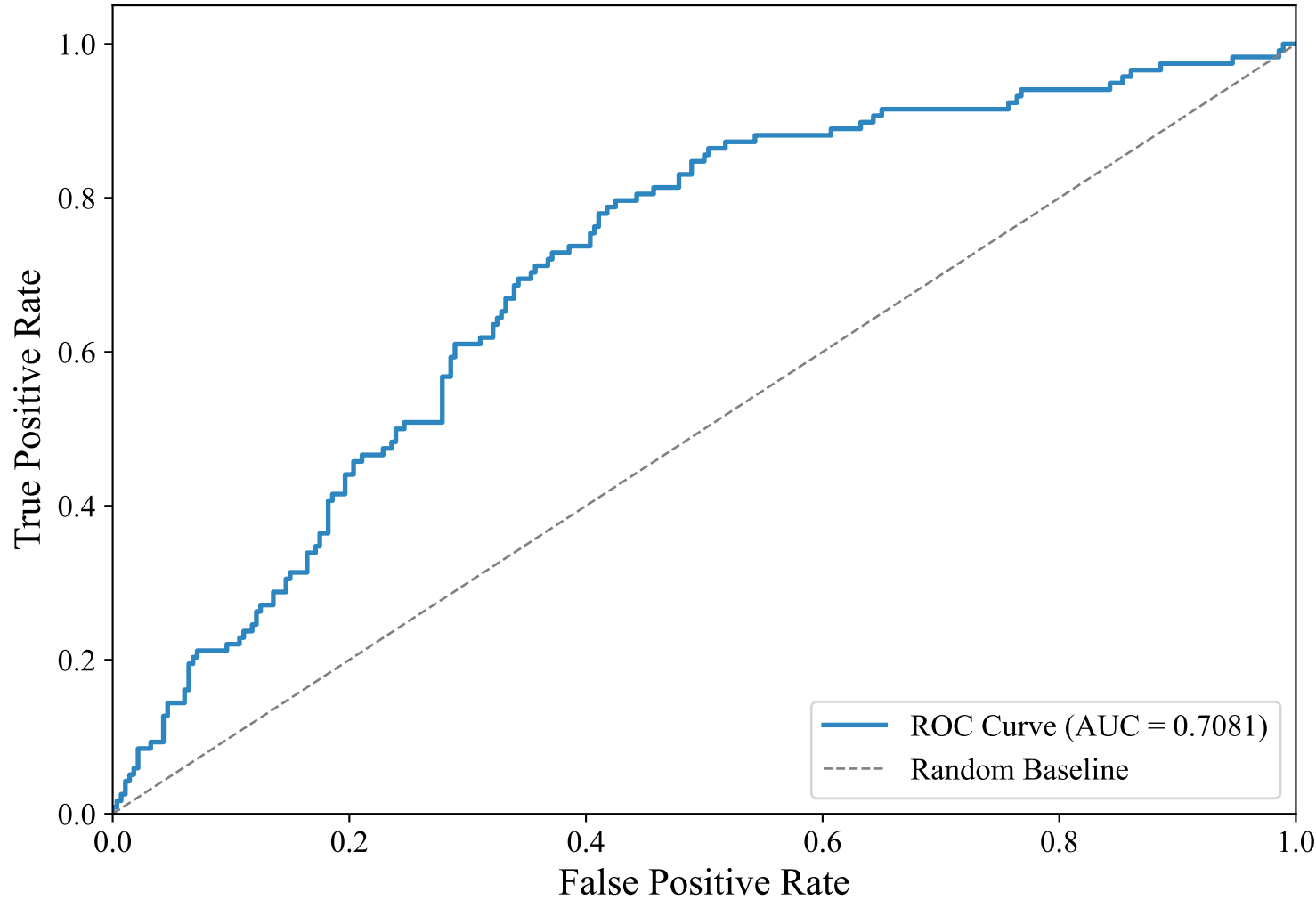
ROC Curve — DUTCH_MANUAL (paraphrase-multilingual-mpnet-base-v2, svm_linear)
