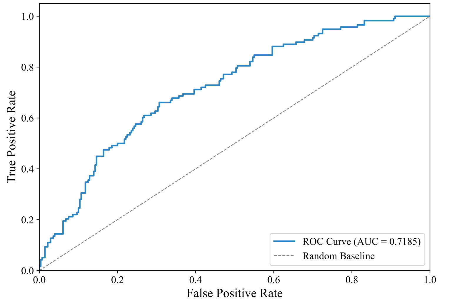
ROC Curve — DUTCH_MANUAL (paraphrase-multilingual-mpnet-base-v2, xgboost)
