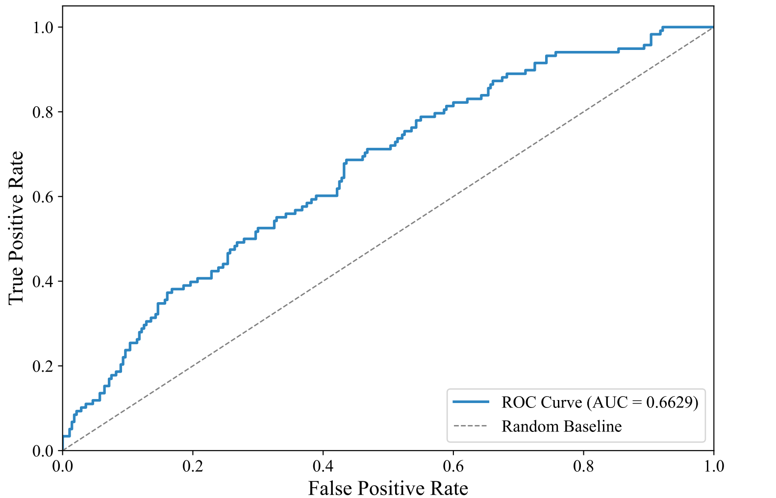
ROC Curve — DUTCH_MANUAL (snowflake-arctic-embed-l-v2.0, random_forest)
