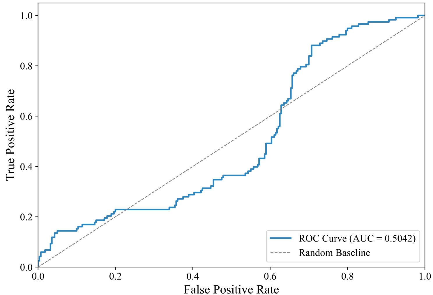
ROC Curve — DUTCH_MANUAL (xlm-roberta-base, lightgbm)
