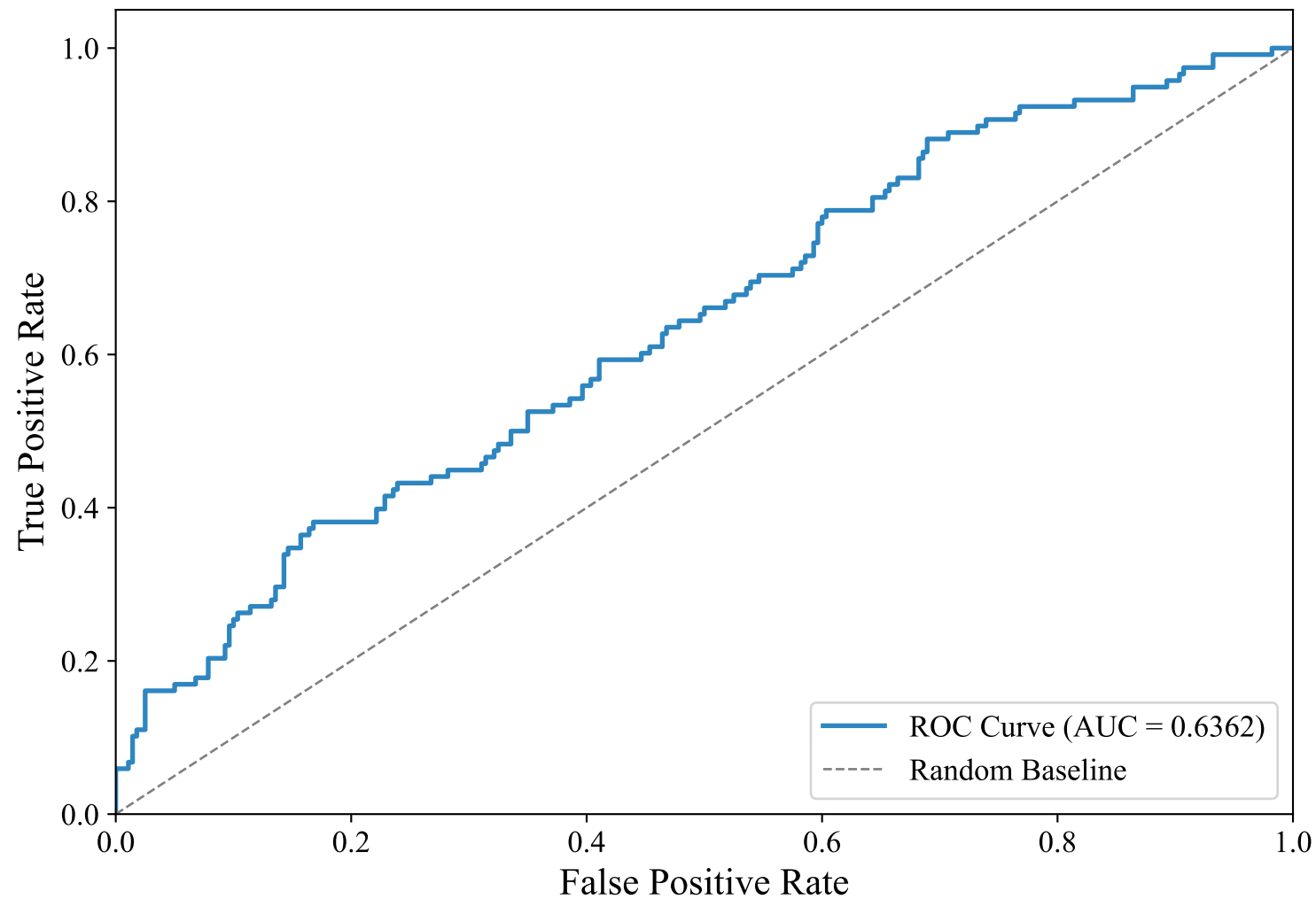
ROC Curve — DUTCH_MANUAL (xlm-roberta-base, random_forest)
