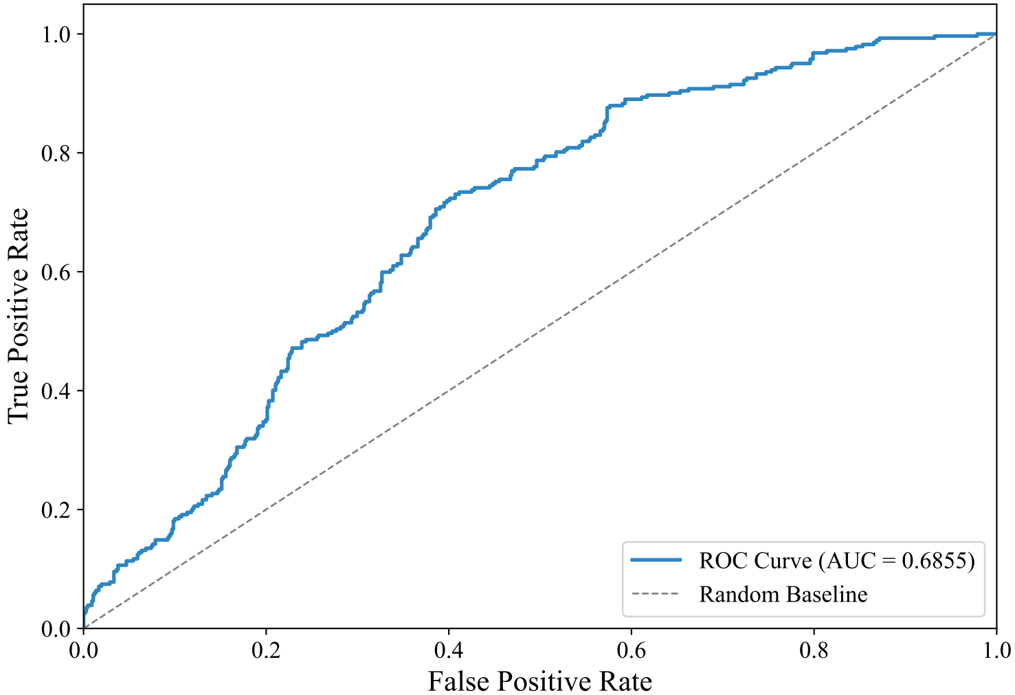
ROC Curve — ENGLISH_MANUAL (bert-base-multilingual-uncased, lightgbm)
