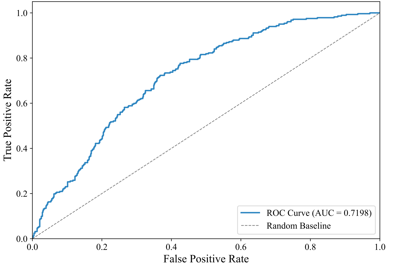
ROC Curve — ENGLISH_MANUAL (bert-base-multilingual-uncased, svm_linear)
