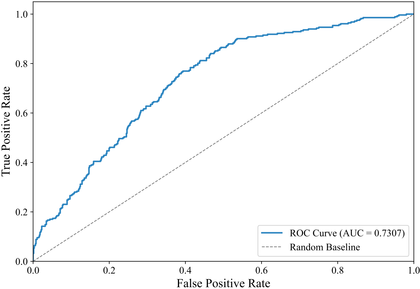
ROC Curve — ENGLISH_MANUAL (multilingual-e5-large-instruct, lightgbm)
