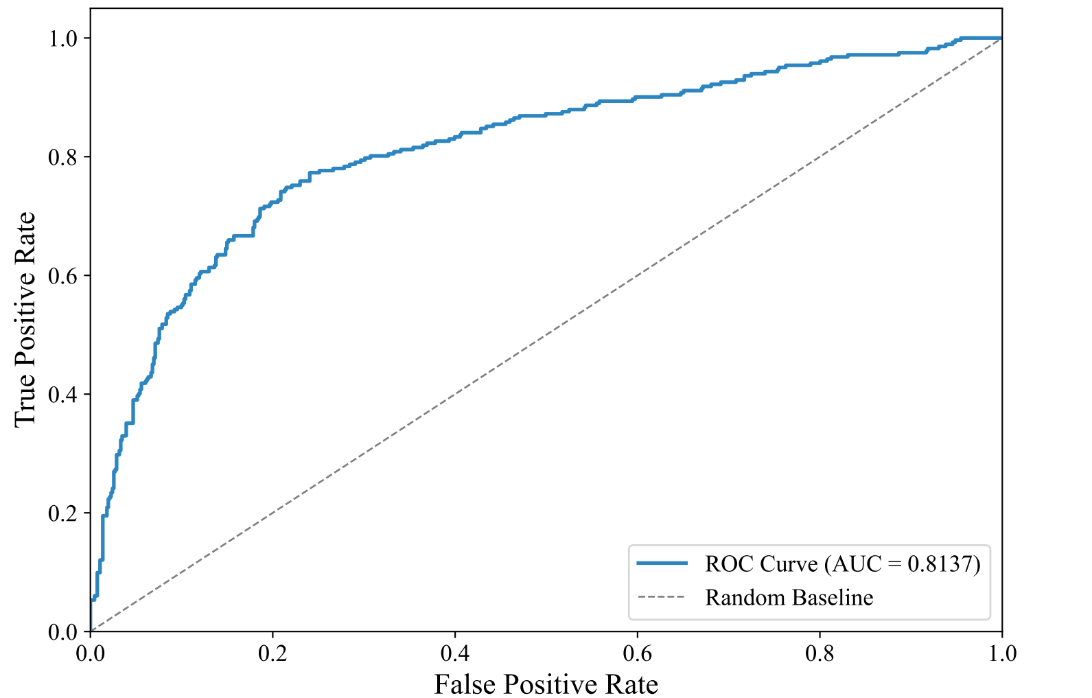
ROC Curve — ENGLISH_MANUAL (paraphrase-multilingual-MiniLM-L12-v2, random_forest)
