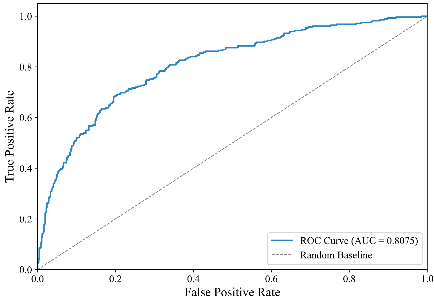
ROC Curve — ENGLISH_MANUAL (paraphrase-multilingual-mpnet-base-v2, lightgbm)
