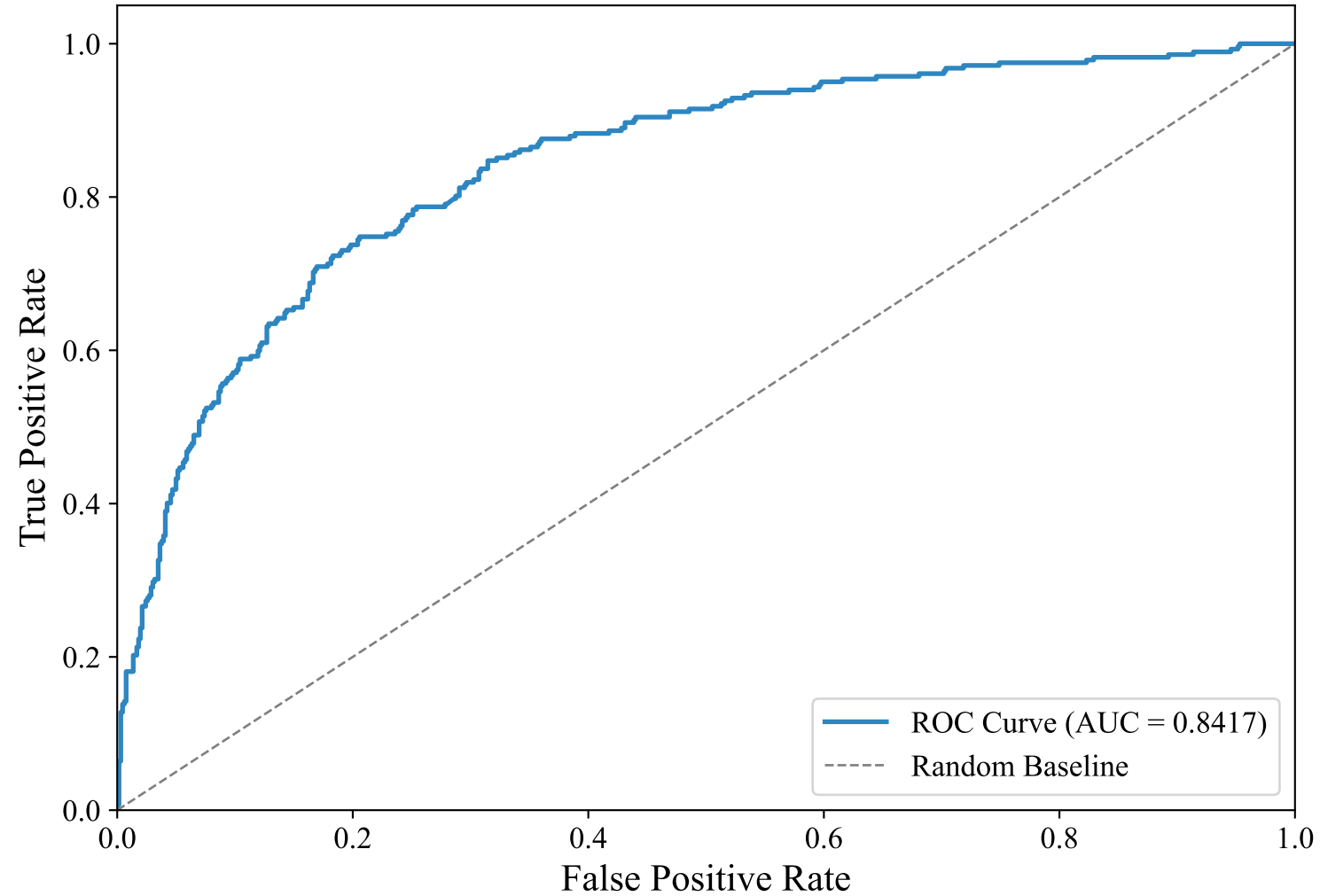
ROC Curve — ENGLISH_MANUAL (paraphrase-multilingual-mpnet-base-v2, svm_rbf)
