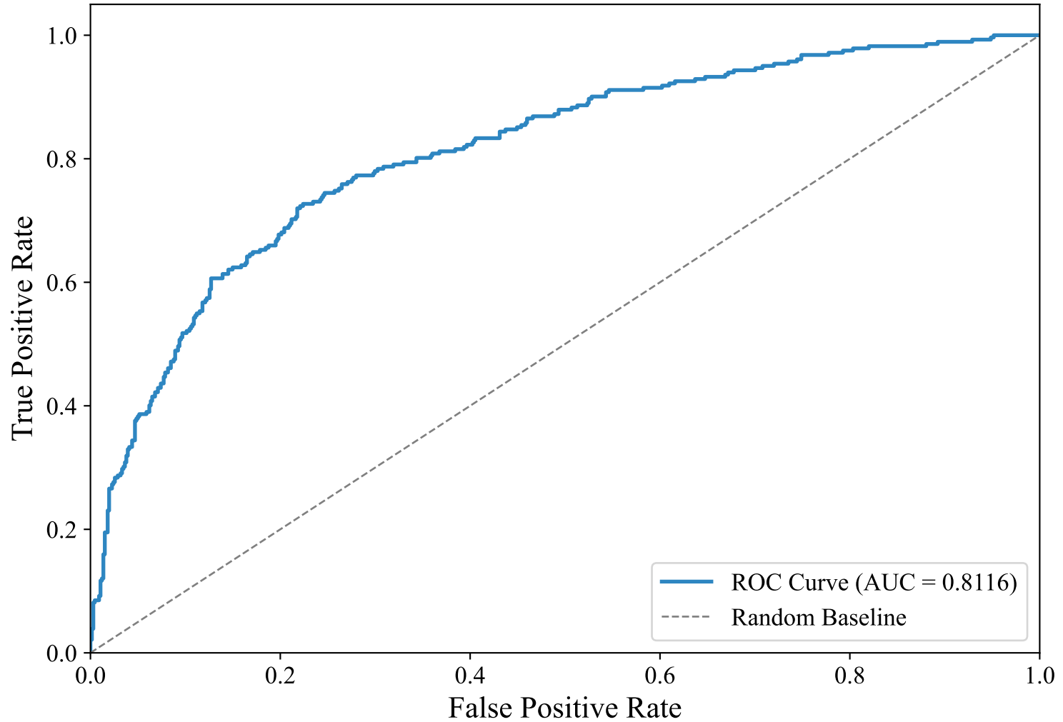
ROC Curve — ENGLISH_MANUAL (paraphrase-multilingual-mpnet-base-v2, xgboost)
