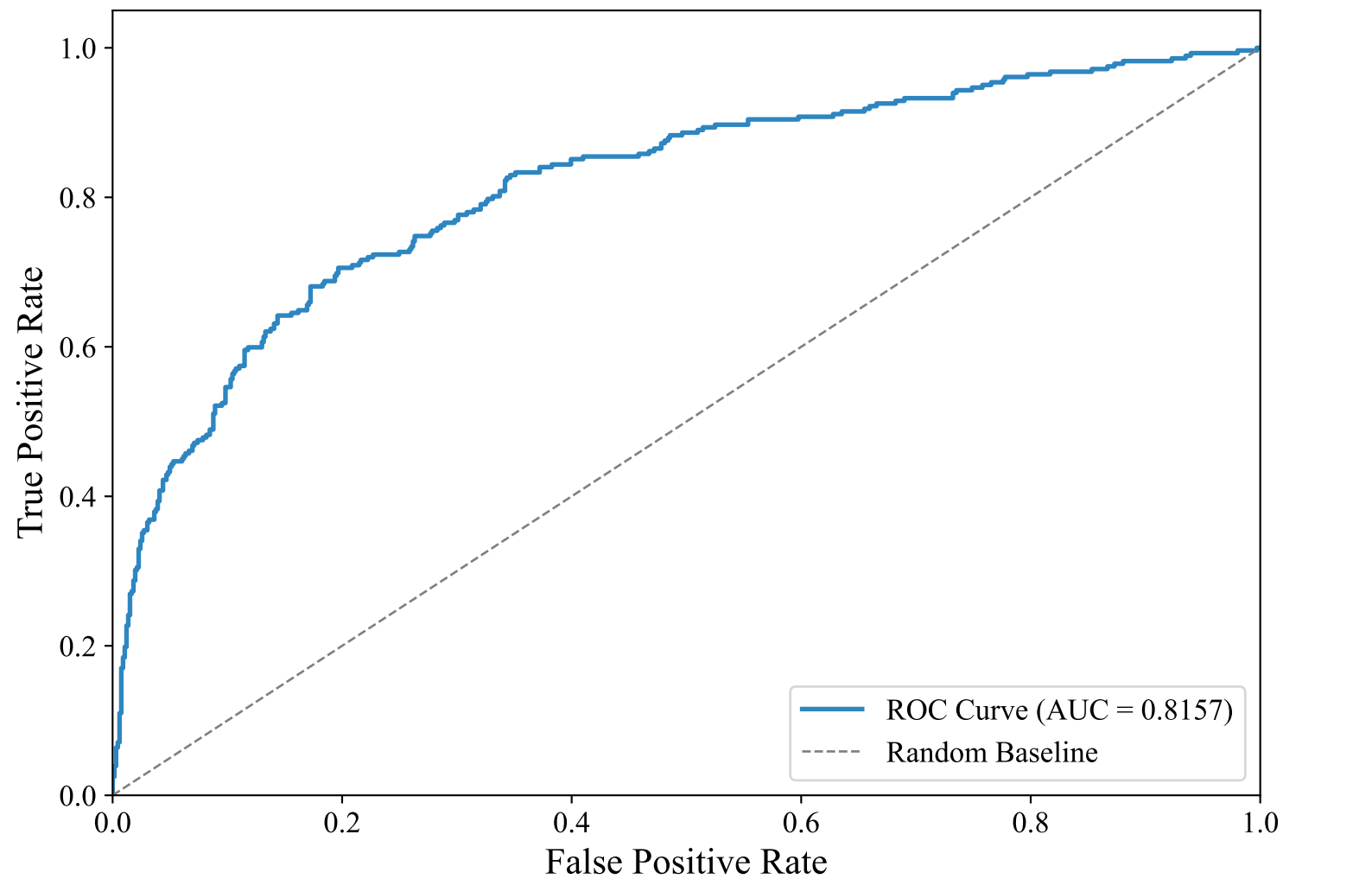
ROC Curve — ENGLISH_MANUAL (snowflake-arctic-embed-l-v2.0, random_forest)
